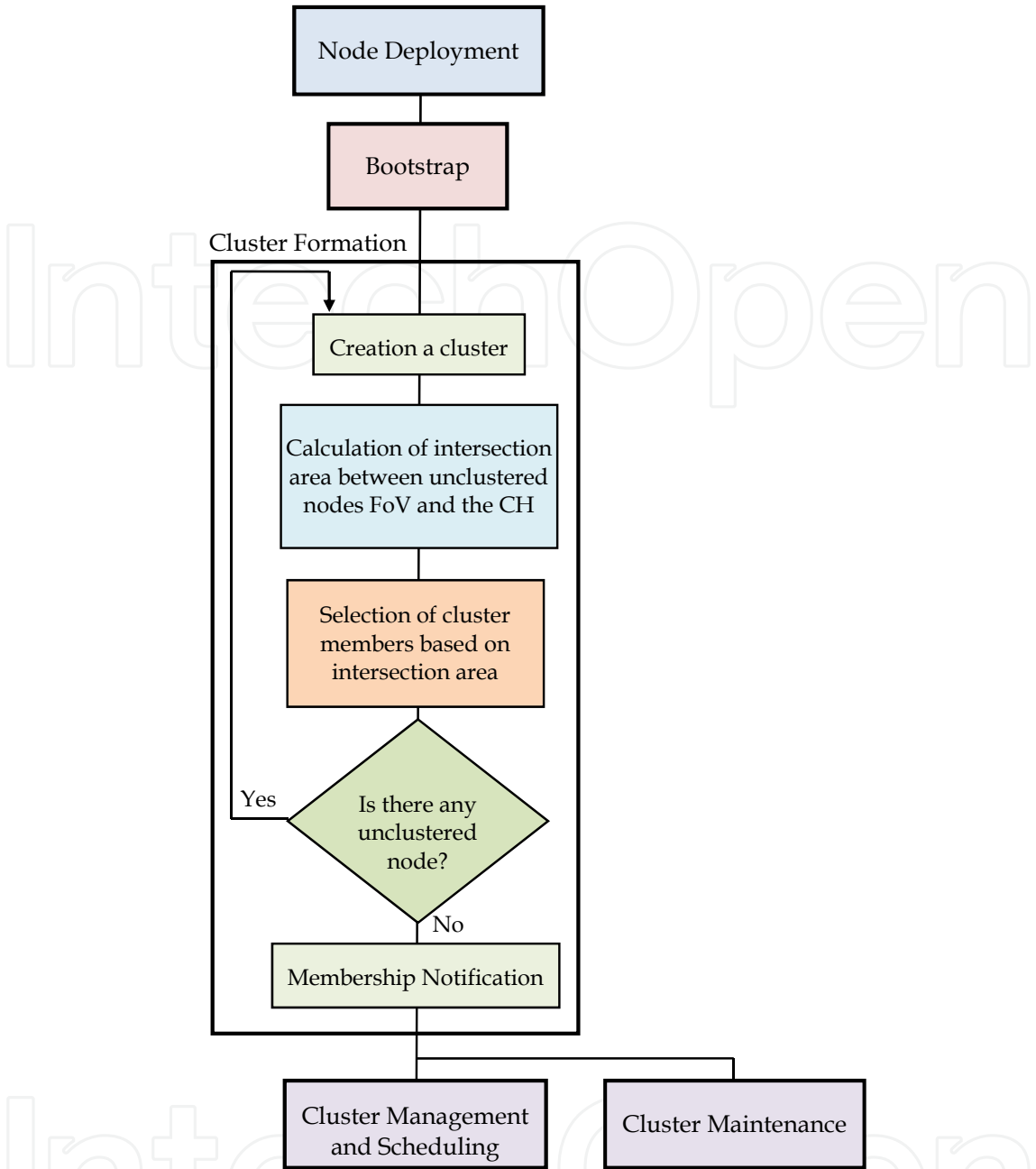
Fig. 2. Clustering Procedure.
