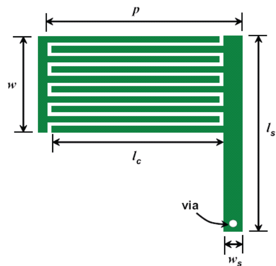
Fig. 37. Layout of a single unit cell of CRLH-TL LWA were p is the length of the unit cell period, l_c , is the length of the capacitor w and w_s represent, the overall width of its finger and the width of the stub respectively.
