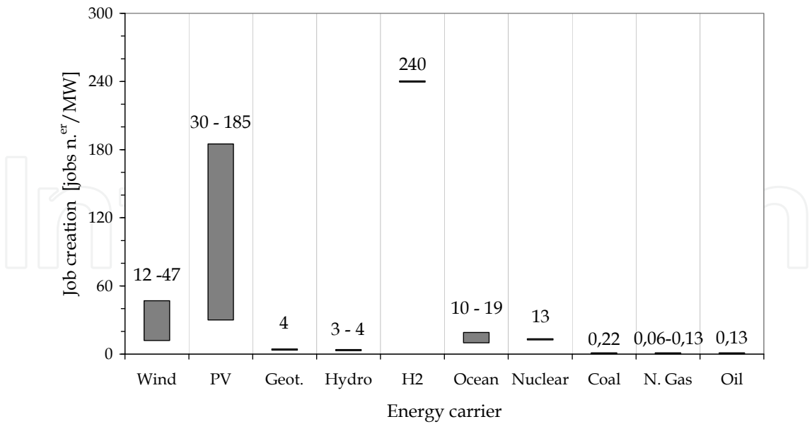
Fig. 9. Values range of job creation (Jobs n. er /MW) for each energy carrier.
