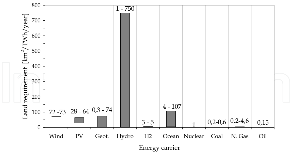
Fig. 8. Values range of land requirements (km²/TWh/year) for each energy carrier.
