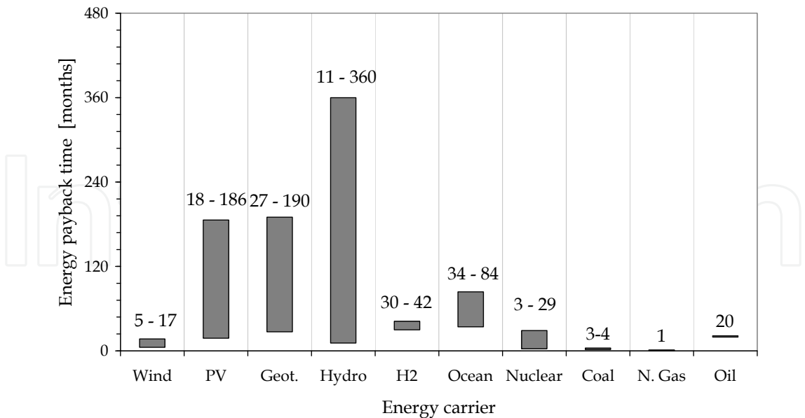
Fig. 4. Values range of energy payback time (months) for each energy carrier.
