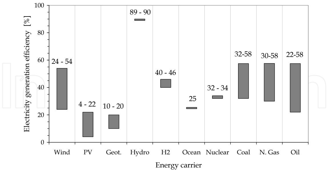
Fig. 2. Values range of electricity generation efficiency (%) for each energy carrier.
