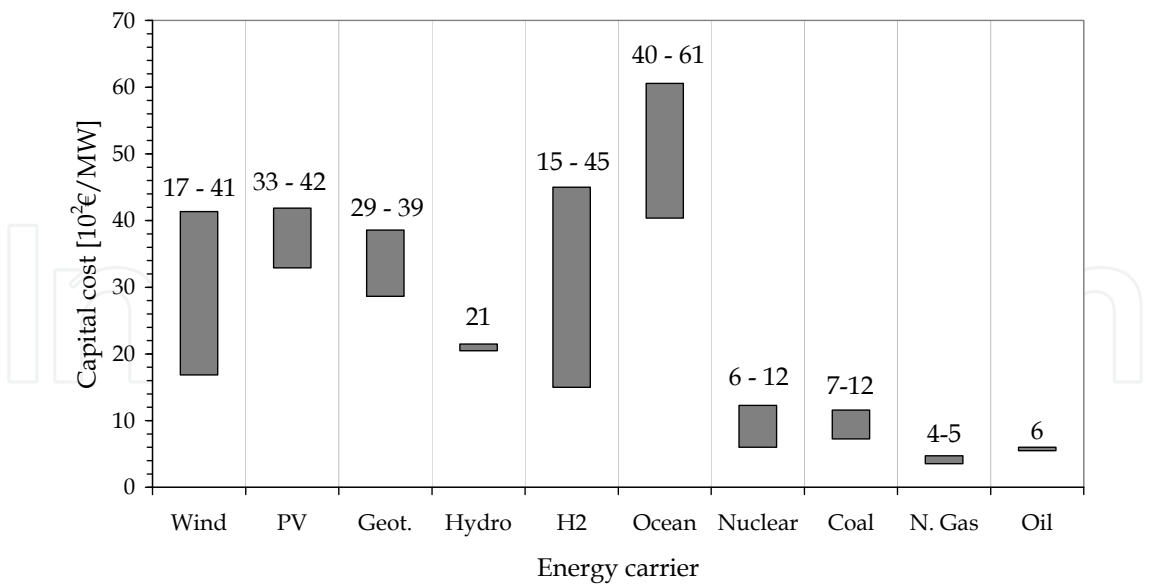
Fig. 5. Values range of capital cost (10²€/MW) for each energy carrier.
