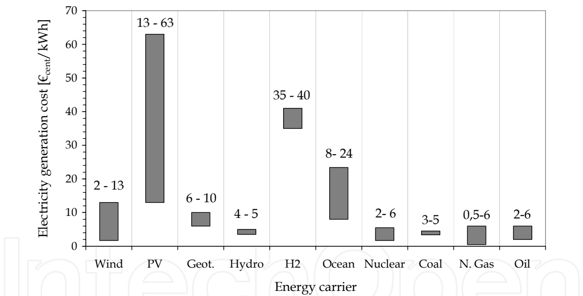
Fig. 6. Values range of electricity generation cost (€/cent/kWh) for each energy carrier.
