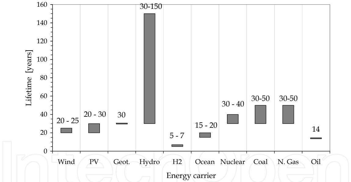
Fig. 3. Values range of lifetime (years) for each energy carrier.
