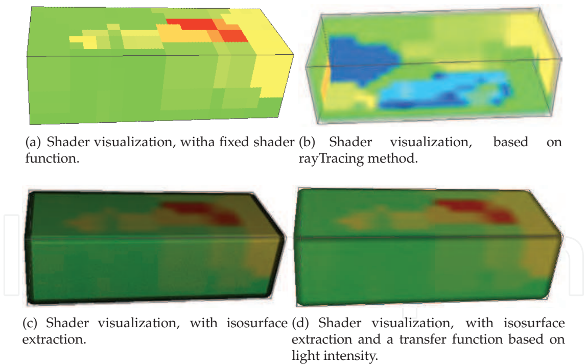
Fig. 16. Real time visualization of particles using shader programming language.
