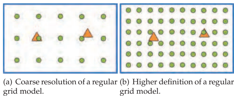
Fig. 3. Regular grid model used to render volume of a room. Dots represent particles, triangles represent sensors. Another possible construction method for particles grid is a concentric pattern. Particles are dropped in rooms with a concentric sphere centered on sensors. Coordinates of these particles can be computed using the following method:
