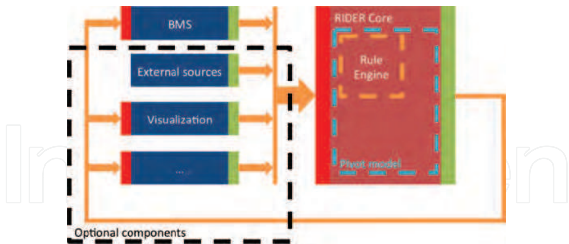
Fig. 1. RIDER architecture.
