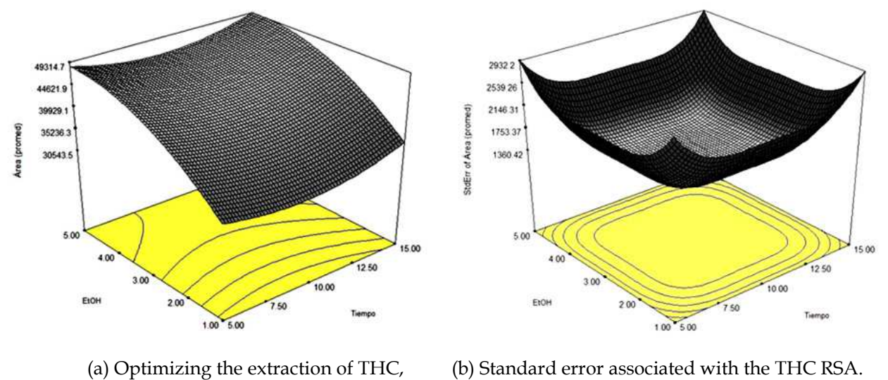
Fig. 3. Response surface analysis (RSA)
