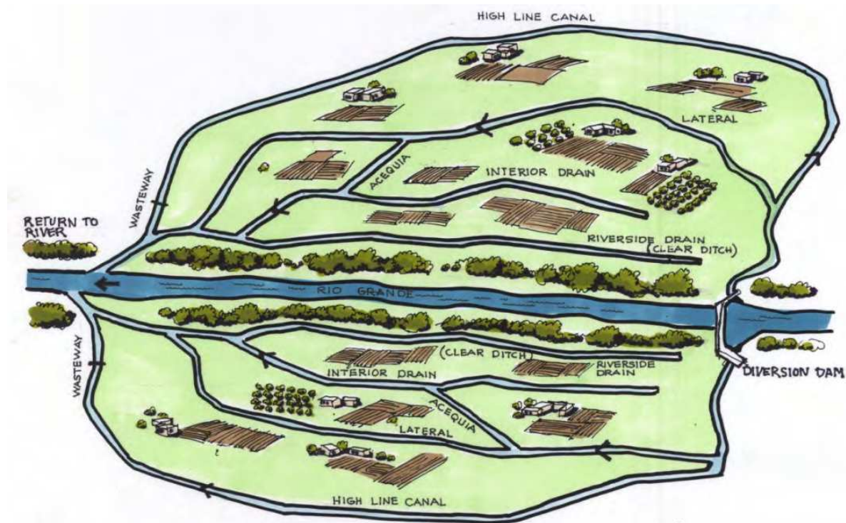
Fig. 2. Representation of MRGCD Irrigation System (Courtesy of David Gensler and MRGCD)
