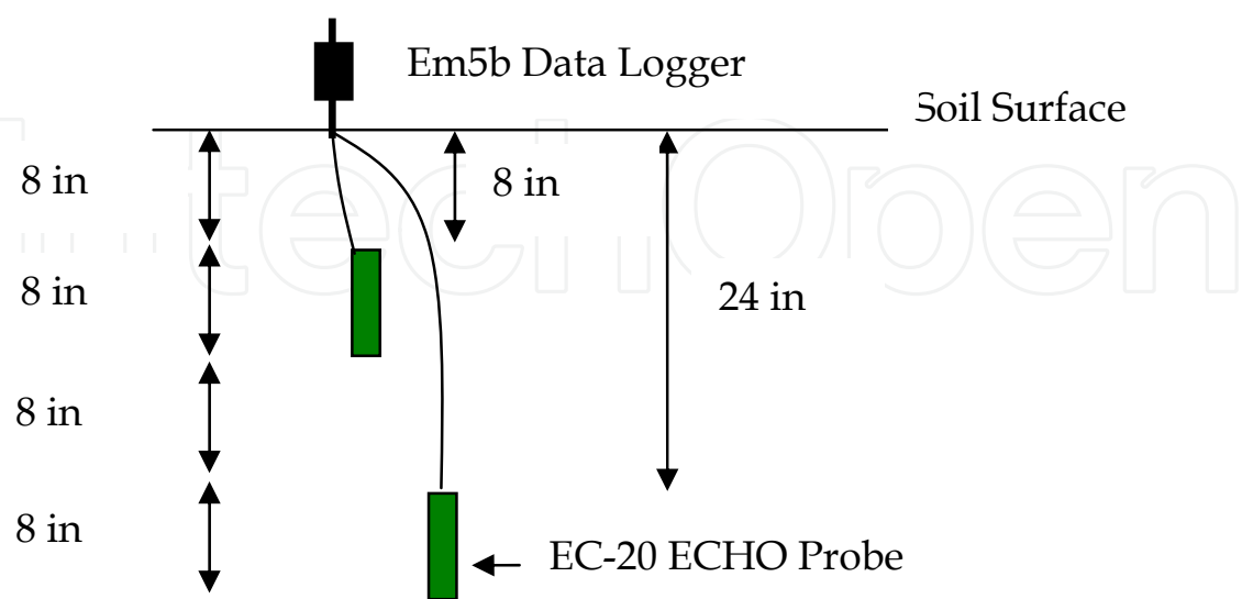
Fig. 11. Individual Layout of Sensor Stations
