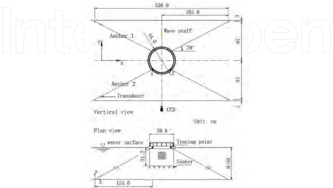
Fig. 8. Arrangement of a gravity cage model in the wave tank
