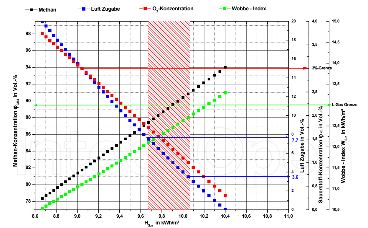
Fig. 6. Possible low calorific L gas mixtures achieved by admixing air to an initial concentration of 94 Vol. -% methane
