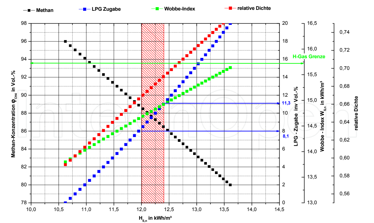
Fig. 3. Possible H gas mixtures by admixing LPG to an initial concentration of 96 Vol. -% methane
