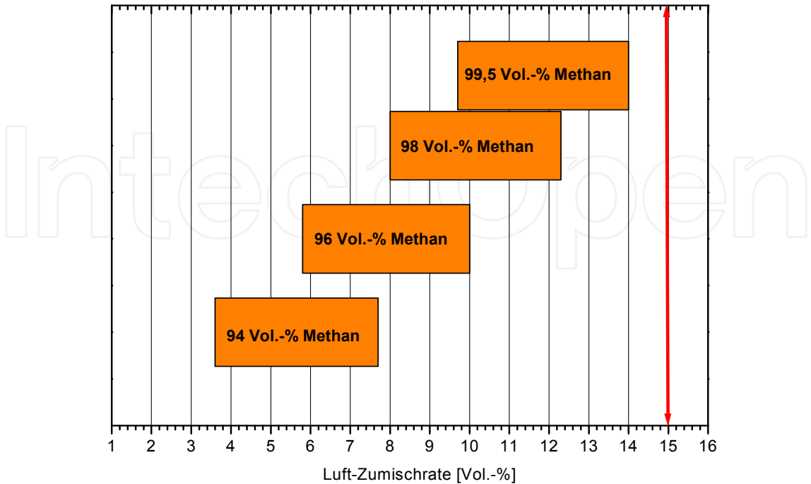
Fig. 8. Rates of air admixture at different initial concentrations of methane
