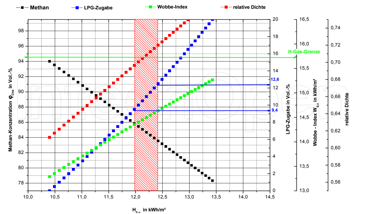
Fig. 2. Possible H gas mixtures by admixing LPG to an initial concentration of 94 Vol. -% methane
