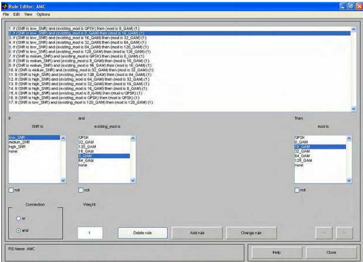
Fig. 15. Rules editor
