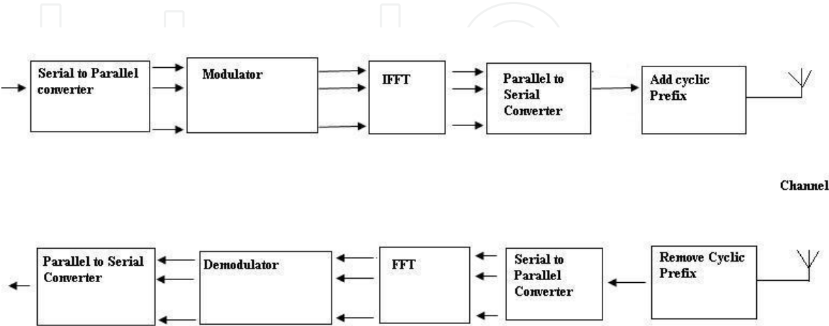
Fig. 1. OFDM system
