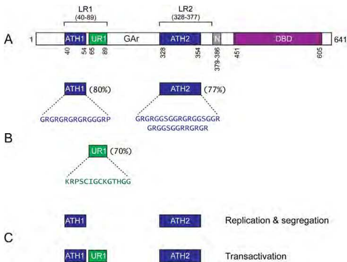
(A) EBNA1 is 641 a.a. in length. ATH1 and ATH2 are two AT-hooks, and UR1 is a domain necessary for transactivation. The GAR is a repeat of glycine and alanine, which can vary in length between EBV isolates. The DBD is used to bind defined sites on EBV's genome. N represents EBNA1's NLS. (B) ATH1 and ATH2 are highly conserved, 80% and 77% respectively, in EBNA1 orthologs from other EBV-like gammaherpesviruses. These regions have a repeated sequence of glycine and arginine. A portion of UR1 is also highly conserved in EBNA1 orthologs. UR1 contains a conserved cys-x-x-cys motif. (C) In addition to DBD, genome replication and segregation requires ATH1 and ATH2. For transactivation, EBNA1 needs both AT-hooks and UR1.
