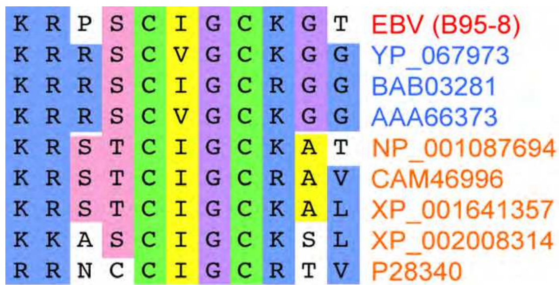
UR1 is highly conserved in the EBNA1 orthologs from other gammaherpesviruses, whose Genbank accession numbers are in blue. The conserved domain closely matches one-half a zinc finger from the DNA polymerase \delta active subunit from many eukaryotic species, whose accession numbers are shown in orange Fig. 5. The UR1 domain of EBNA1.
