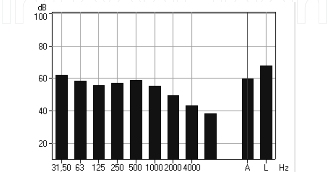
Fig. 13. L_{Leq} graph in octave bands measured in a classroom and used in the simulation of the STI
