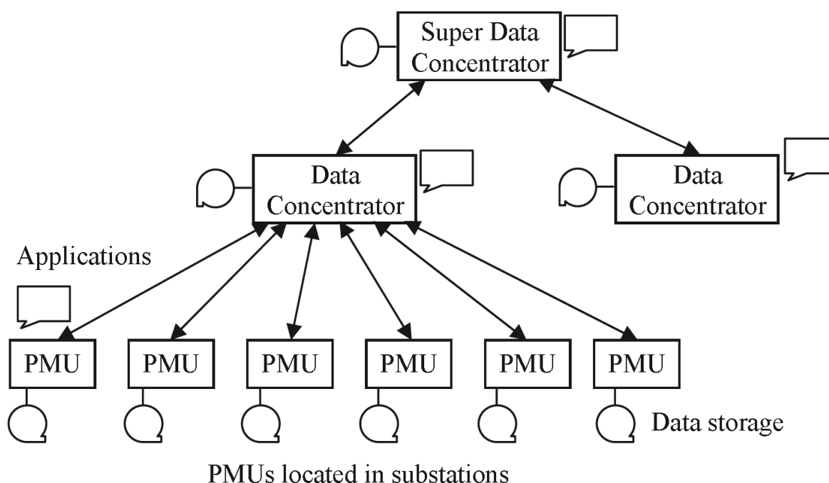
Fig. 3. SPMS sub-systems (Phadke & Thorp, 2008).
