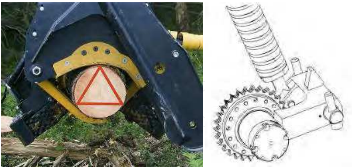
Fig. 2. Photo + scheme of scanning the stem diameter and length at harvesters (both figures according to Ponsse).
