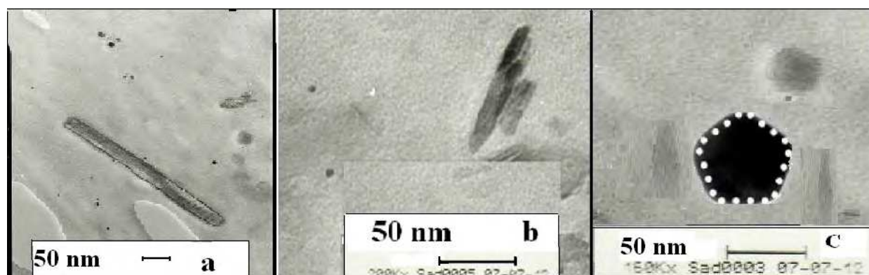
Fig. 2. Transmission electron microscopy (TEM) images of (a,b) individual and (c) cross section of Ag/PVA nanorods.
