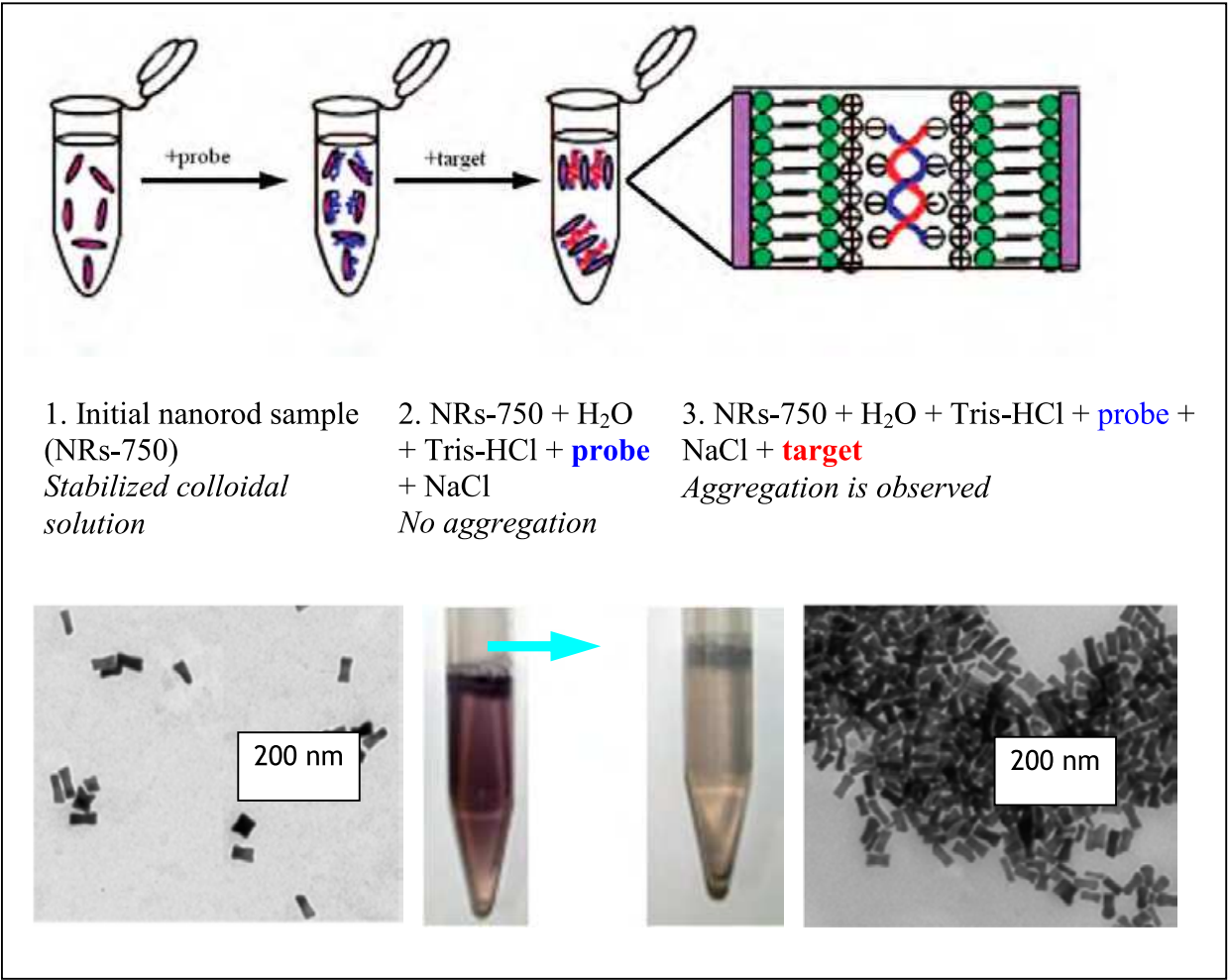
Fig. 7. Experimental diagram for oligonucleotide detection
