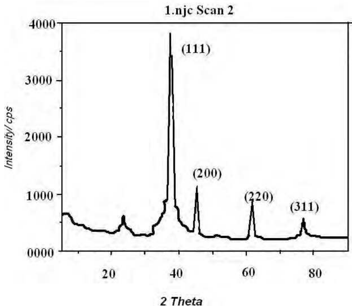
Fig. 4. XRD pattern of Ag/PVA nanocomposite indicative the face-centered cube structure.
