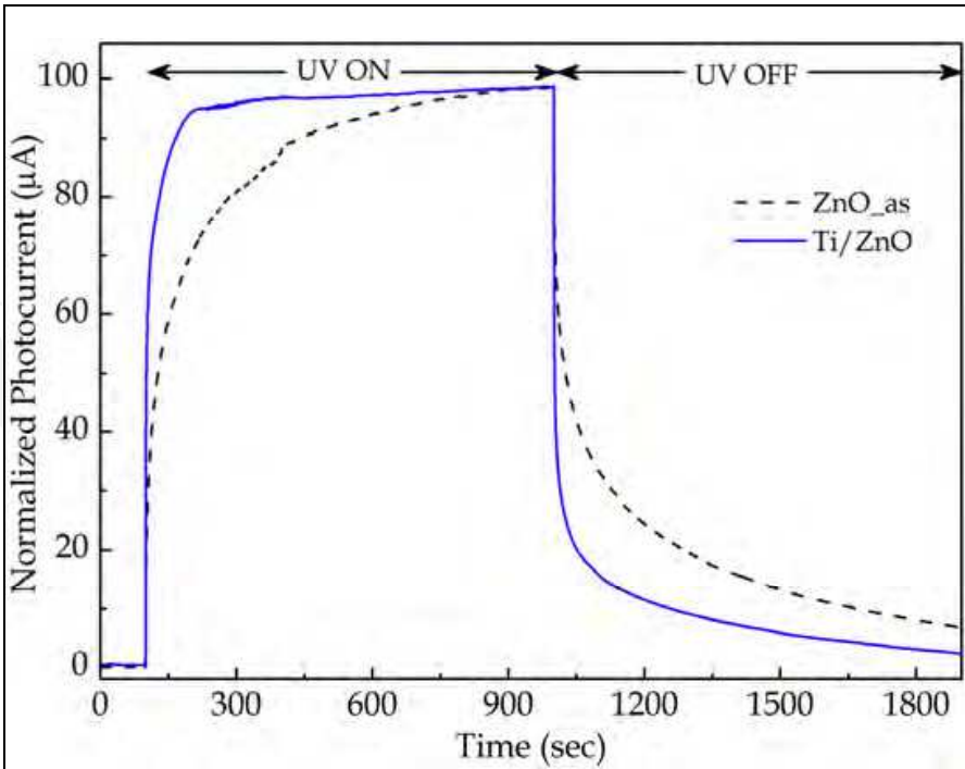
Fig. 22. Photoresponse behaviours of the as-grown NRs and Ti NPs decorated Ti/ZnO NRs heterostructure under the illumination of 365 nm UV light.
