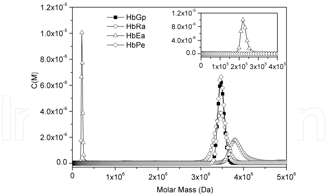
Fig. 5. Continuous molecular mass distribution of extracellular hemoglobins. The c(M) fittings for hemoglobins, at a concentration of 300 µg/mL, in 100 mmol/L Tris-HCl containing 50 mmol/L NaCl are shown. The insert shows the enhanced plot in the MM range from 0 to 400 kDa. The MM for each fitted curve was determined as the maximum of the peaks of c(M) curves. Absorbance was monitored at 415 nm.
