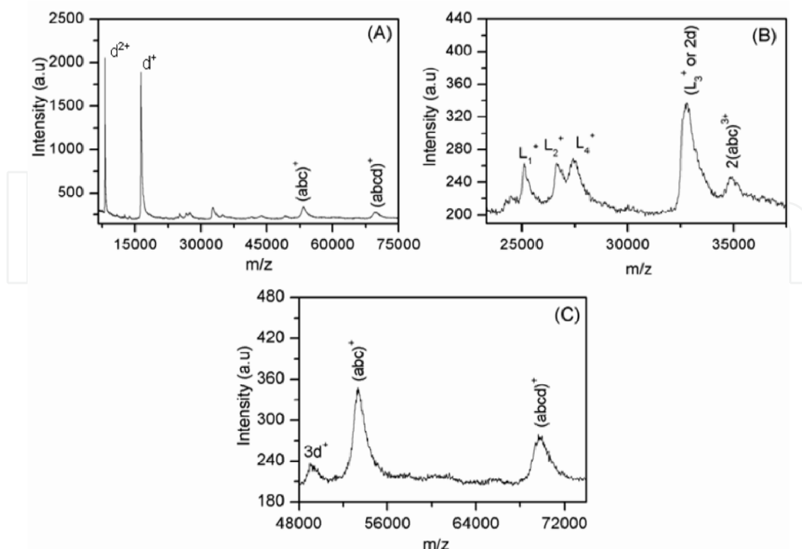
Fig. 3. MALDI-TOF-MS spectrum of Eisenia andrei hemoglobin, HbEa. (A) at pH 7.0, full mass range. (B) Corresponds to the intensity in arbitrary units, highlighting the linkers and triple-protonated dimer of trimer; (C) the expanded region for the mono-protonated trimer abc^+ and tetramer abcd^+ from 48,000 to 75,000 Da.
