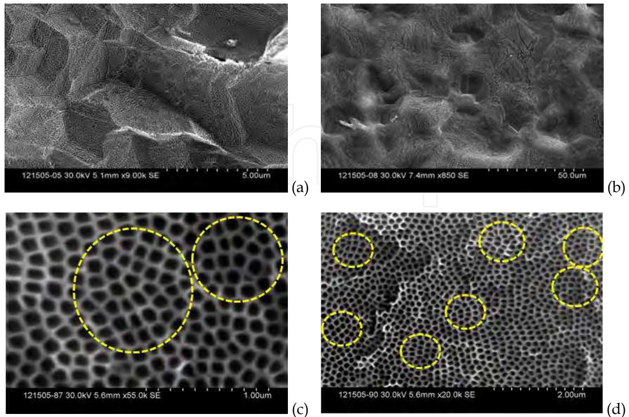
Fig. 10. SEM images of \text{TiO}_2 NTs under 5 hrs anodization on etched Ti substrate. (a) anodized surface at higher magnification; (b) anodized surface at lower magnification; (c) highly ordered NT with local concavity shown highlighted in yellow circle; (d) several concave geometries highlighted in yellow circles
