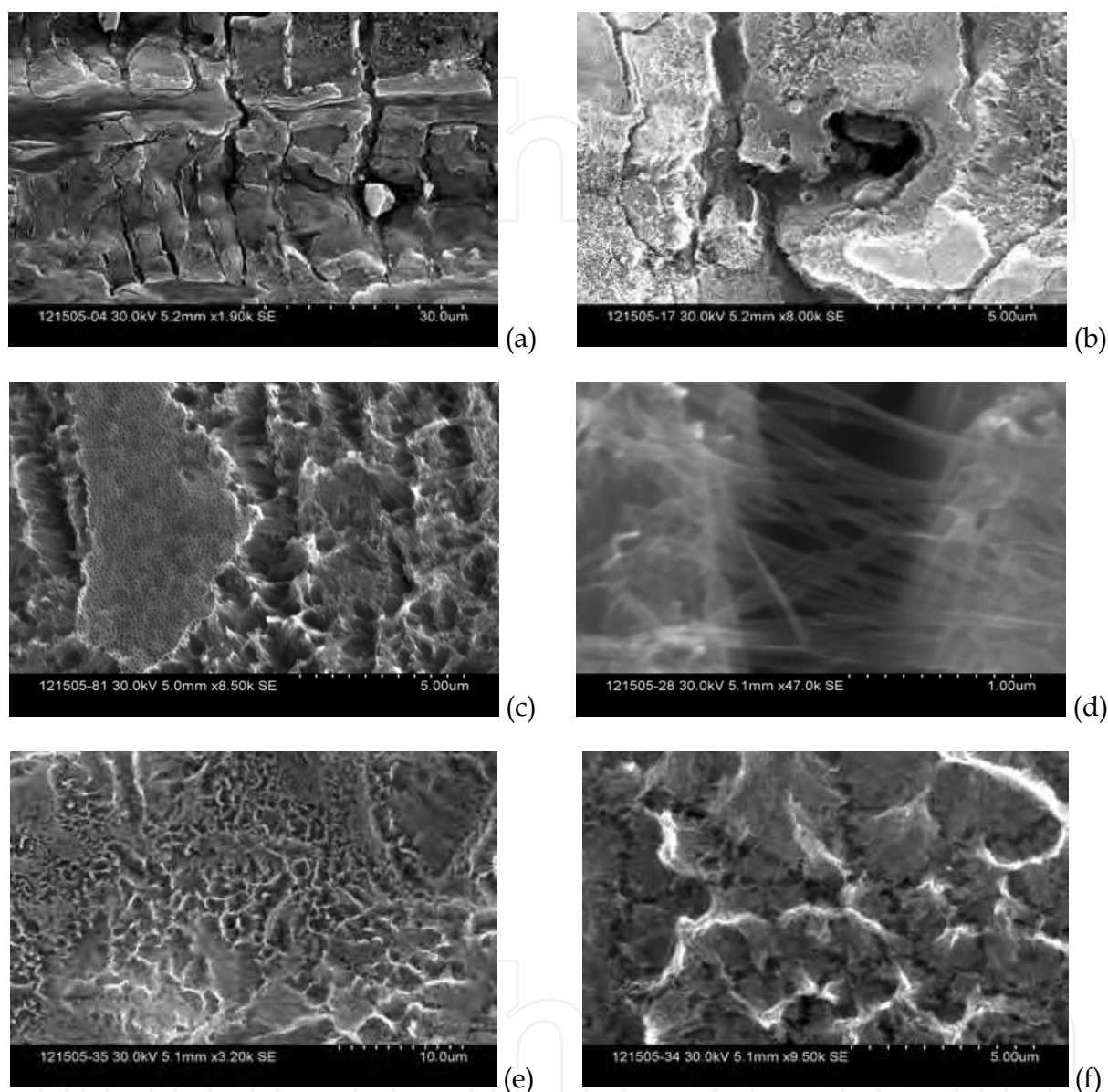
Fig. 6. (a) \text{TiO}_2 NTs after 30 min anodization; (b) \text{TiO}_2 NT with a whirlpool geometry at crack site; (c) \text{TiO}_2 NT cluster formed at crack lines; (d) Collapsed \text{TiO}_2 NTs at crack lines; (e) \text{TiO}_2 bundles throughout sample and (f) \text{TiO}_2 bundles under higher magnification
