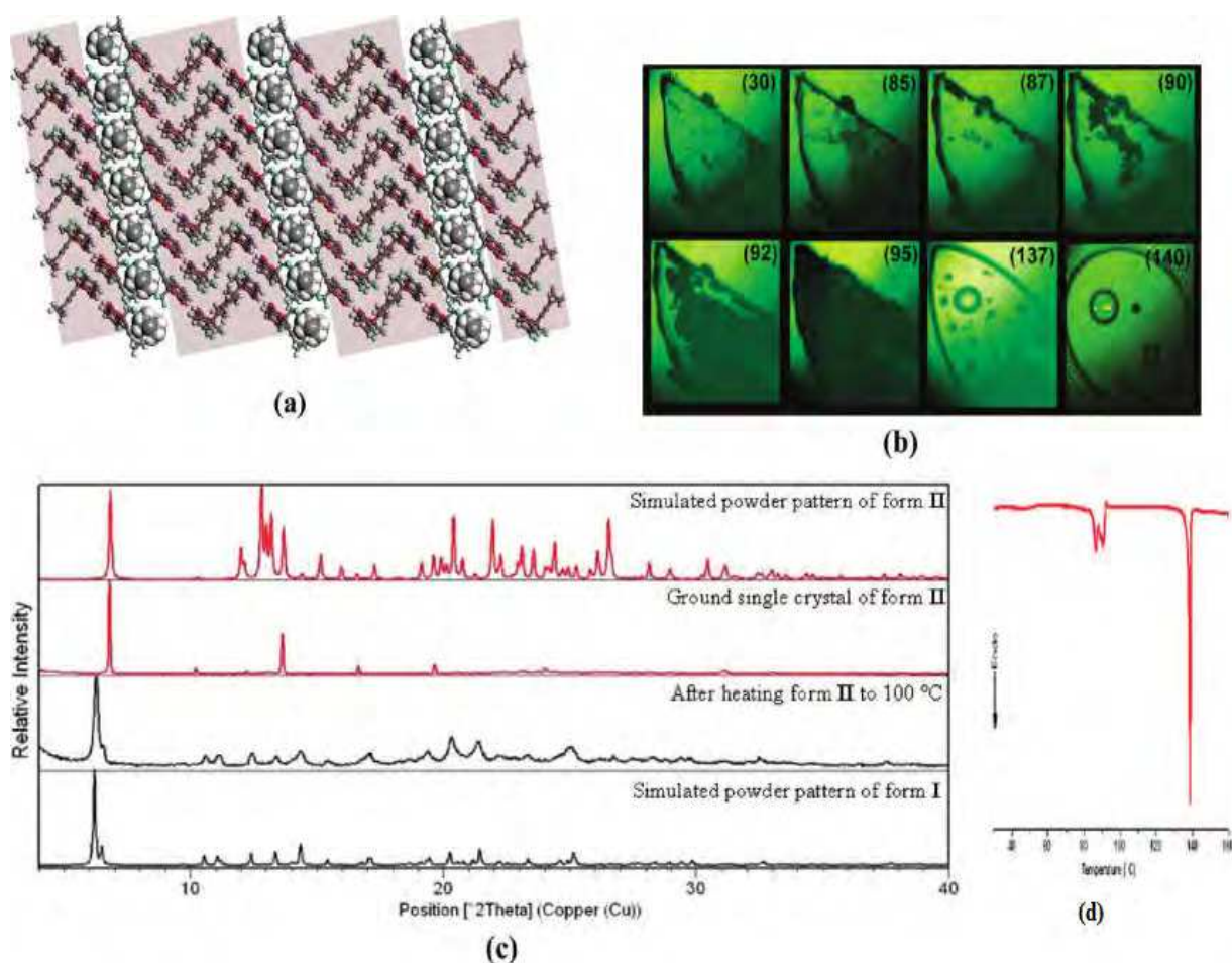
Fig. 8. (a) Crystal packing of efavirenz with the guest cyclohexane molecules represented in the space filling mode (b) HSM images of II (corresponding temperatures are given in parentheses) (c) PXRD patterns of forms I and II and the heated sample of form II (d) DSC plot for form II.
