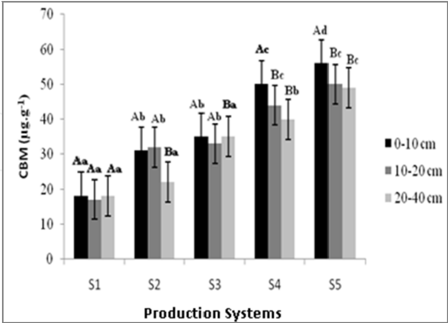
Fig. 4. Values of microbial biomass carbon (CMB) in different production systems.
