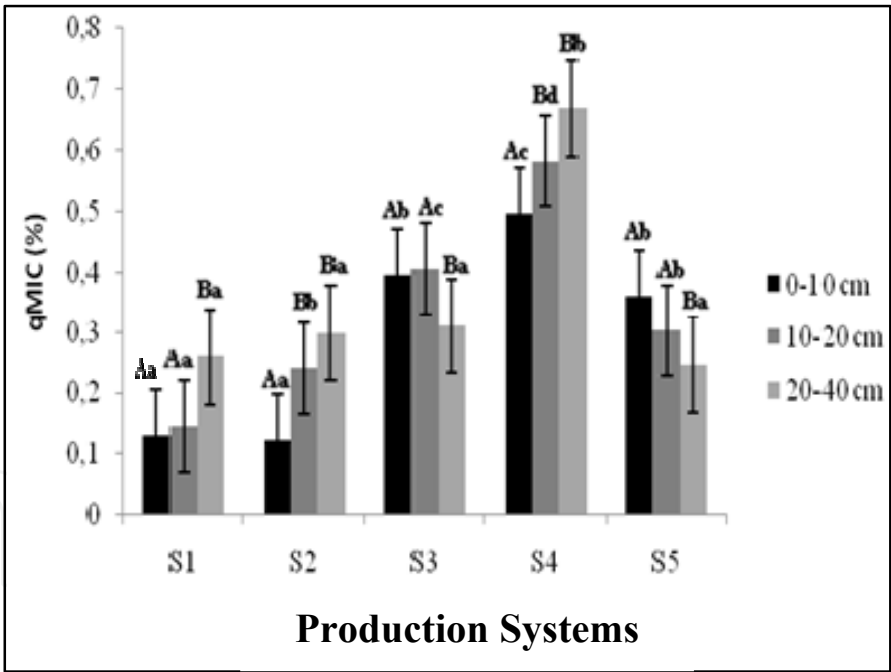
Fig. 5. Values of microbial quotient (qMIC) in different production systems.
