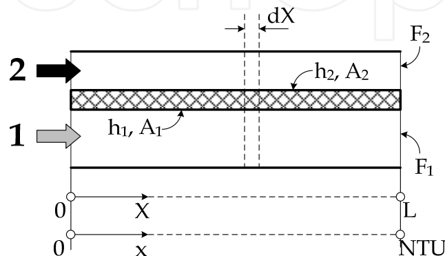
Fig. 1. Schematic Description of Parallel Flow Heat Exchanger.
