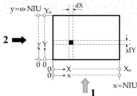
Fig. 3. Schematic Description of Cross Flow Heat Exchanger.
