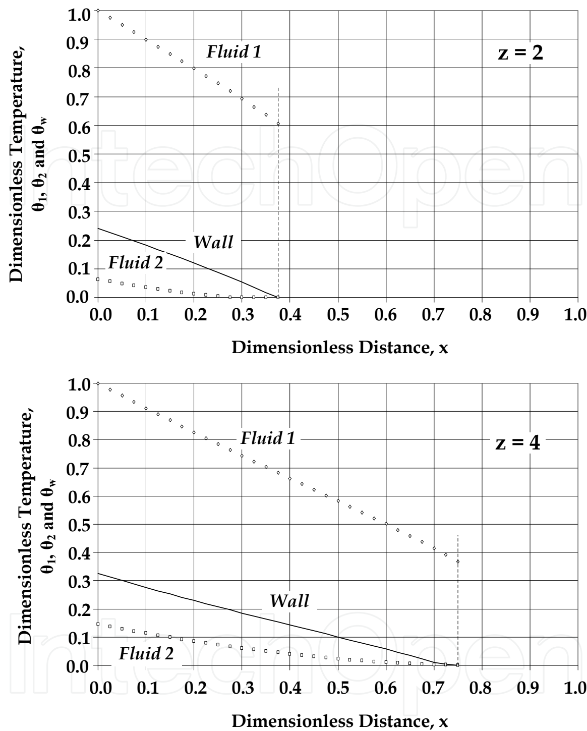
Fig. 5. Temperature Distribution of Both fluids and the Wall of Counter Flow Heat Exchanger for z = 2 and 4 .
