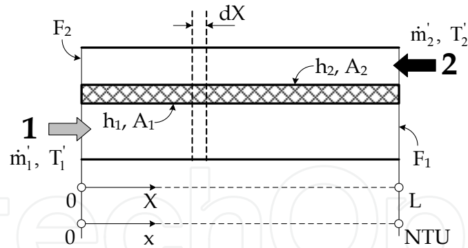
Fig. 2. Schematic Description of Counter Flow Heat Exchanger
