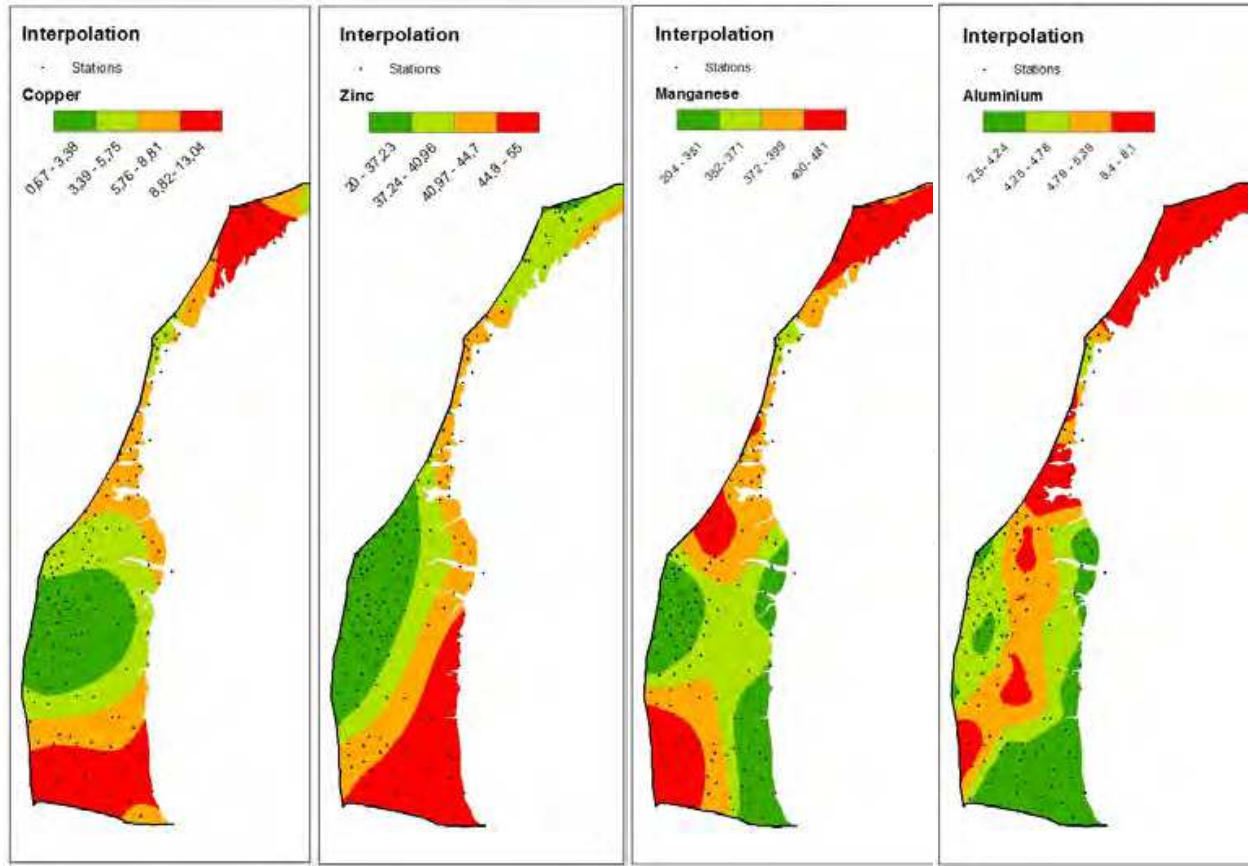
Fig. 15. Spatial distribution of copper, zinc, manganese and aluminium. Values are given in mg kg -1 dry weight, except for Al (in percent)
