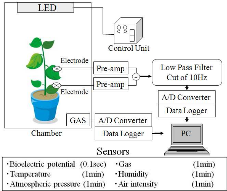
(b) Schematic diagram of the system
