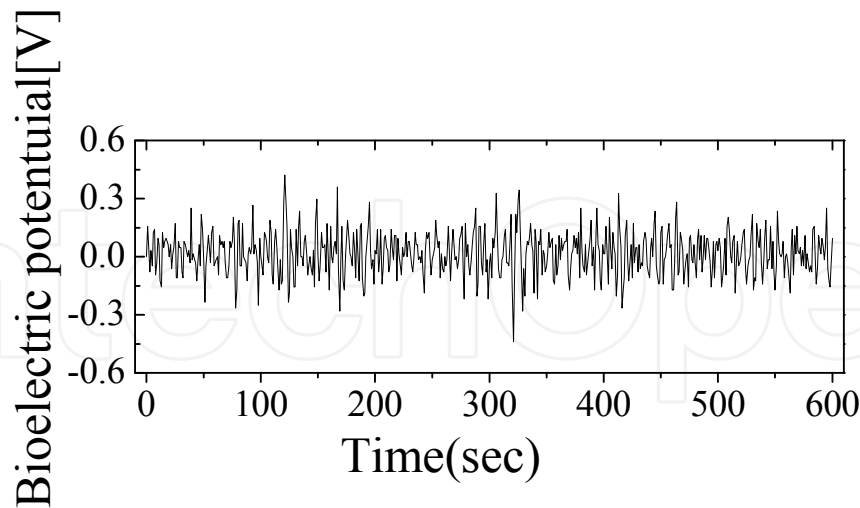
Fig. 2. Original characteristic of bioelectric potential for pothos
