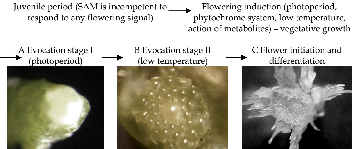
Fig. 1. Model of flowering initiation.
