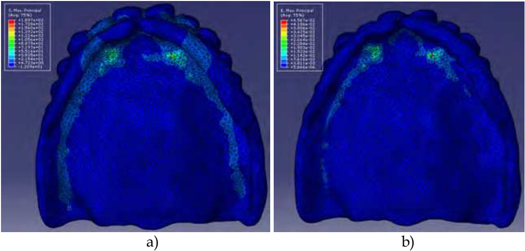
Fig. 21. The Maximum Principal Stress (a) and Maximum Principal Strain (b) state in the third analysis model for denture with Eclipse material
