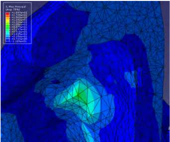
Fig. 22. The Maximum Principal Stress around the defect in the third analysis model for denture with Eclipse material
