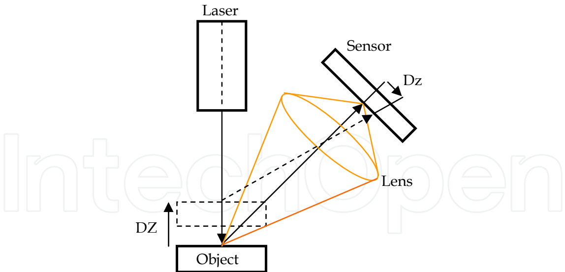
Fig. 2. Principle of laser triangulation sensor
