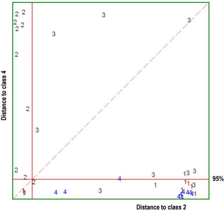
Fig. 14. Cooman's plot for the classes 2 and 4.
