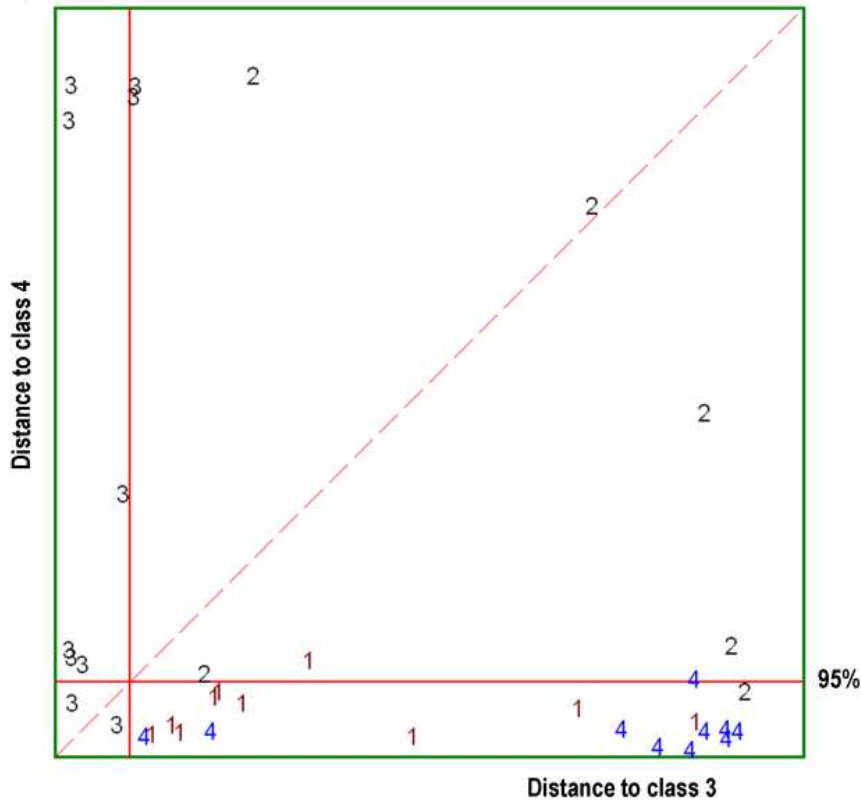
Fig. 15. Cooman's plot for the classes 3 and 4.
