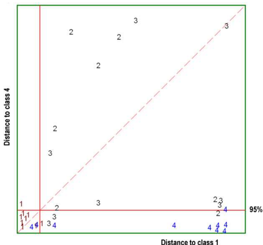
Fig. 13. Cooman's plot for the classes 1 and 4.
