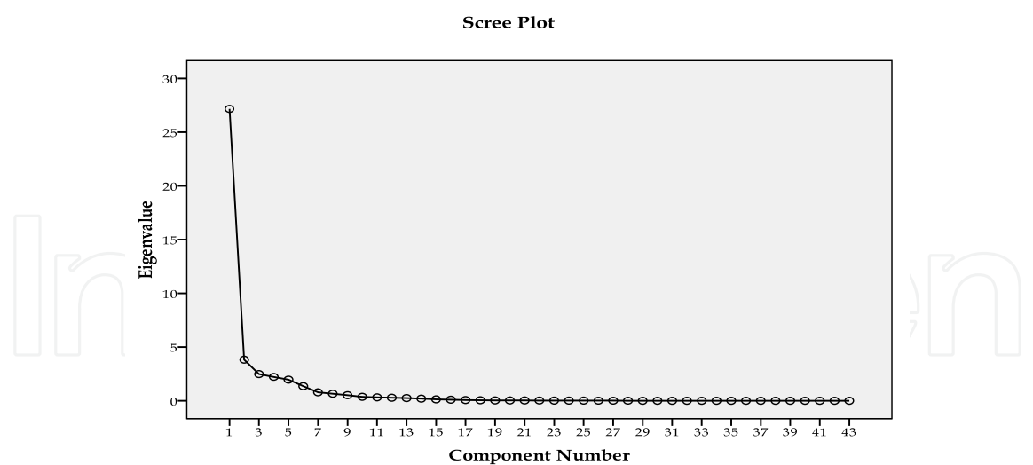
Fig. 10. Scree plot for the low level data fusion
