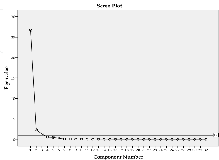
Fig. 3. Illustration of the scree plot.
