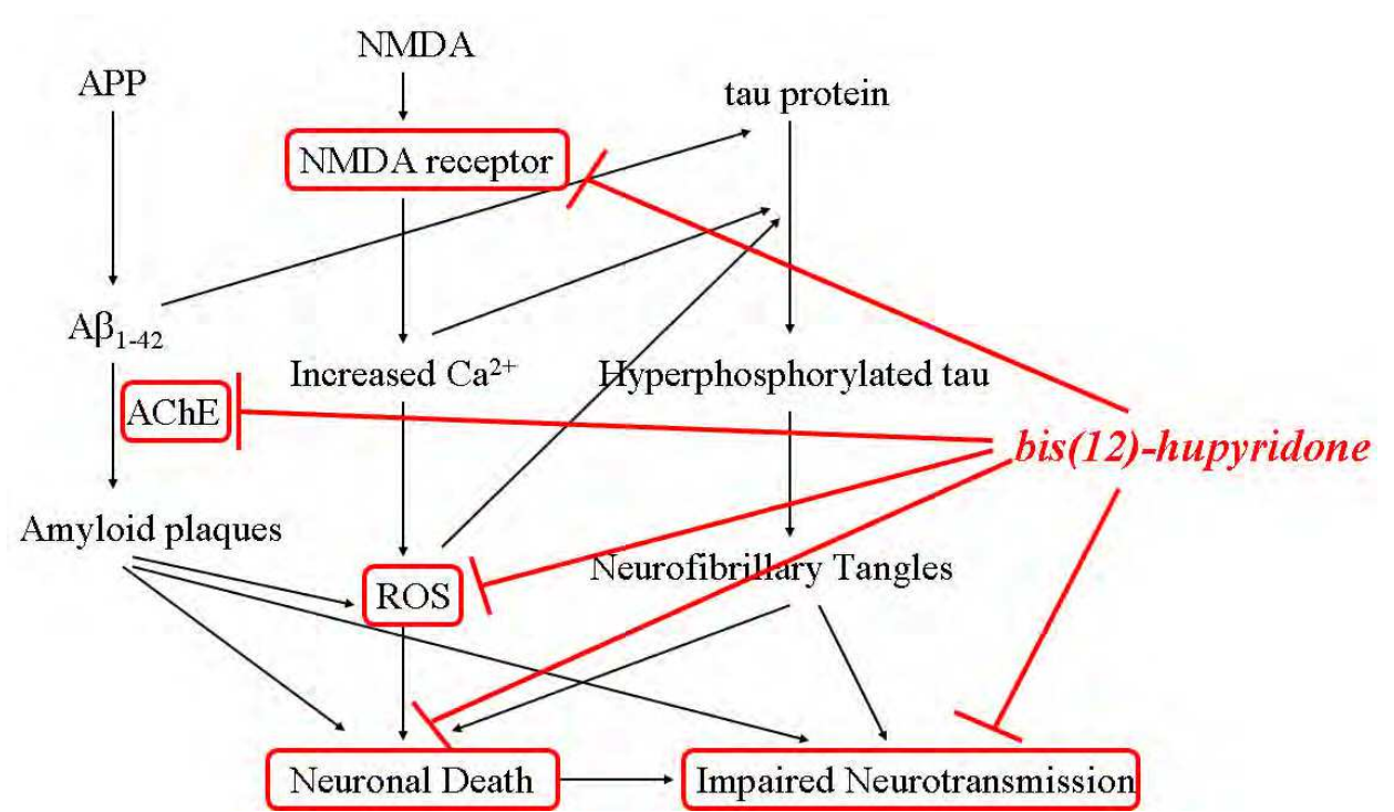
Fig. 10. Bis(12)-hupyradone acts as a multi-functional dimer for the treatment of AD.
