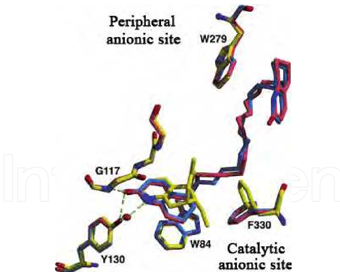
Fig. 3. Overlay of the refined structures of TcAChE /(-)-bis(10)-hupyrindone (sky blue), TcAChE /(-)-bis(12)-hupyrindone (pink), and TcAChE /(-)-huperzine A (yellow). Inhibitors and protein residues are rendered as sticks, and water molecules are shown as red spheres. The figure is modified from the reference (Wong et al., 2003).
