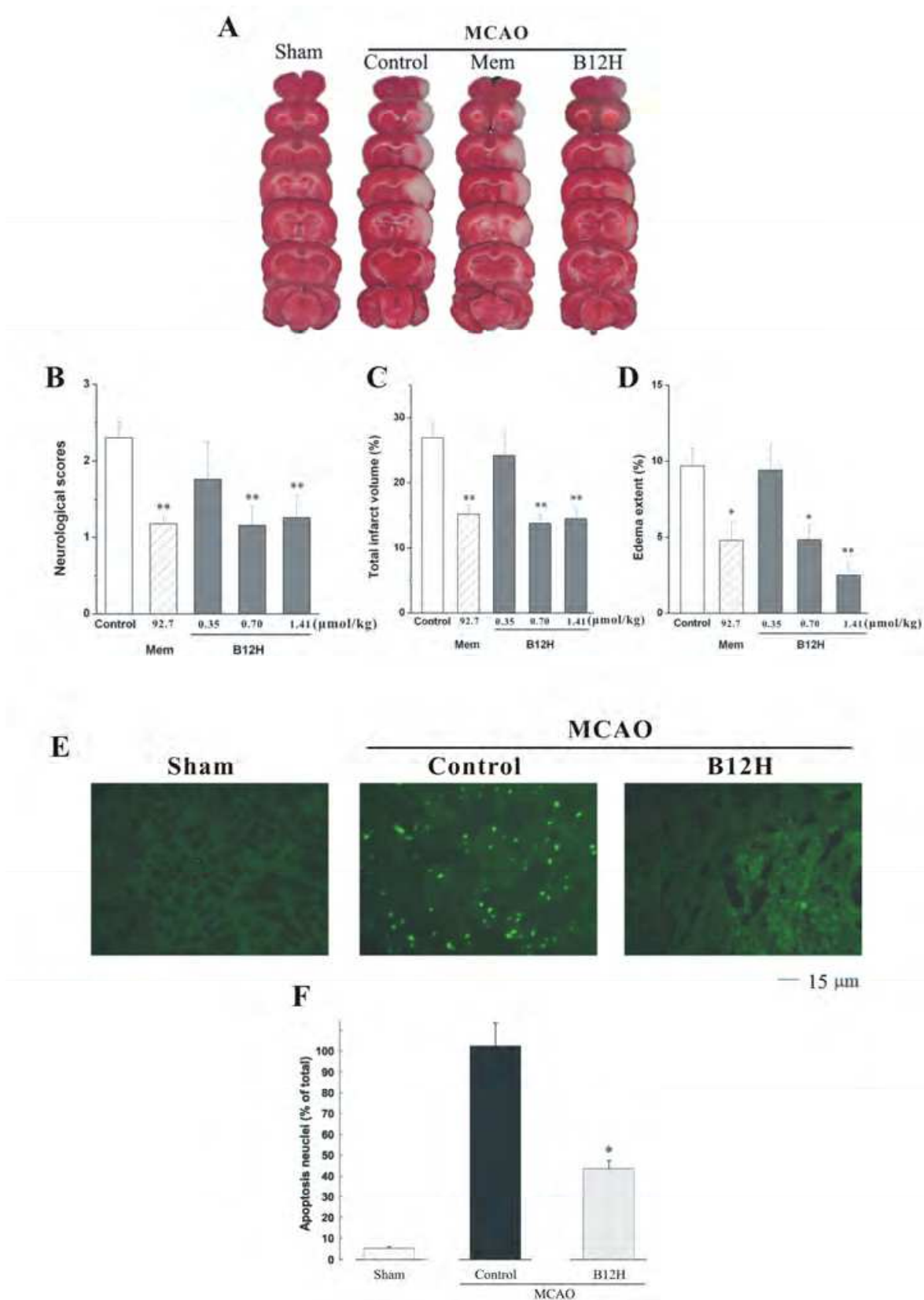
Fig. 9. Bis(12)-hupyrindone rescues acute neurological impairments in rats after 2 h of MCAO followed by 24 h of reperfusion. Bis(12)-hupyrindone was injected i.p. 30 min pre-ischemia and 15 min post-ischemia. (A) Representative photos of 2, 3, 5-triphenyltetrazolium
