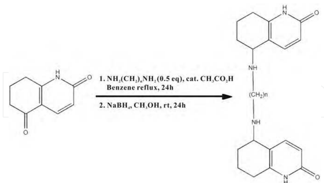
Fig. 2. Synthesis of bis(n)-hupyrindones.
