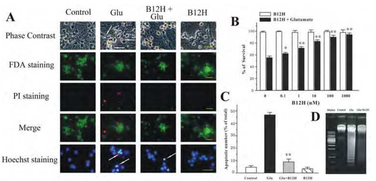
Fig. 4. Bis(12)-hupyrindone prevents neuronal death induced by glutamate in primary CGNs. (A) CGNs were pre-incubated with or without 1 \mu M bis(12)-hupyrindone and exposed to 75 \mu M glutamate 2 h later. At 24 h after glutamate challenge, CGNs were assayed with a phase contrast microscope, fluorescein diacetate/propidium iodide double staining and Hoechst 33324 staining. Apoptotic nuclei were indicated by white arrows. (B) CGNs were pre-incubated with bis(12)-hupyrindone at different concentrations as indicated and exposed to 75 \mu M glutamate 2 h later. Cell viability was measured by MTT assay at 24 h after glutamate challenge. (C) The counts of apoptotic bodies by Hoechst staining. (D) Under the same treatment conditions as (B), DNA fragmentation was extracted from CGNs after 24 h of challenge, and then agarose gel electrophoresis and ethidium bromide staining were used to visualize the DNA extracted from the above samples. B12H: bis(12)-hupyrindone; Glu: glutamate. All data, expressed as percentage of control, were the means \pm SEM of three separate experiments; * p < 0.05, ** p < 0.01 versus glutamate group (ANOVA and Dunnett's test).
