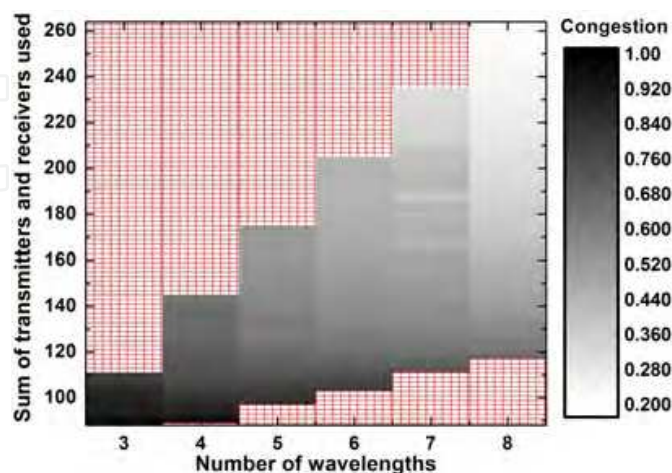
Fig. 14. Fitness of the solutions found by GAPDELT
