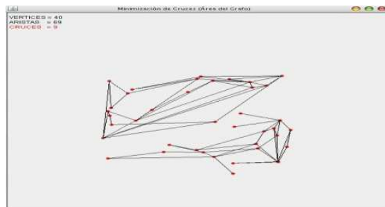
Fig. 17. Generation 500, graph 17470
