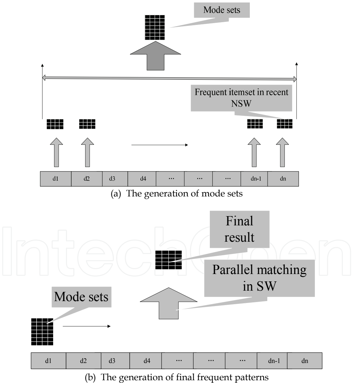
Fig. 6. The process of obtaining frequent patterns
