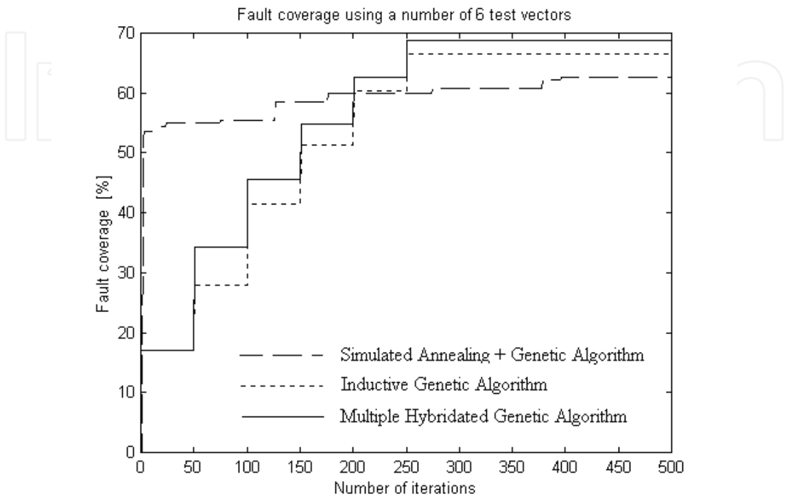
Fig. 7. Fault Coverage Problem of 50 possible faults solved with three HGAs in 500 iterations
