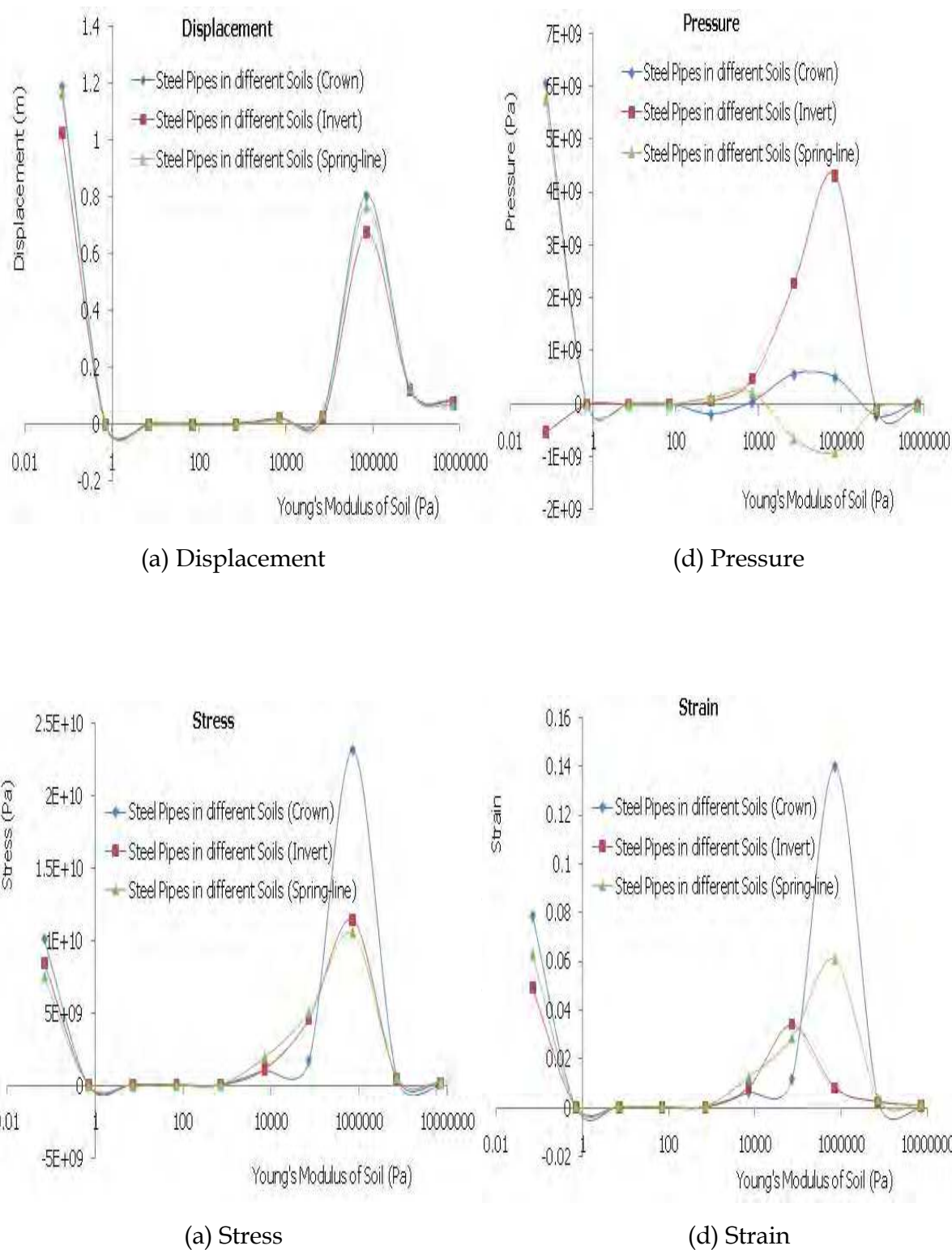
Fig. 7. Displacement, Pressure, Stress and Strain in buried pipes for varying Young's modulus of soil for surface blast
