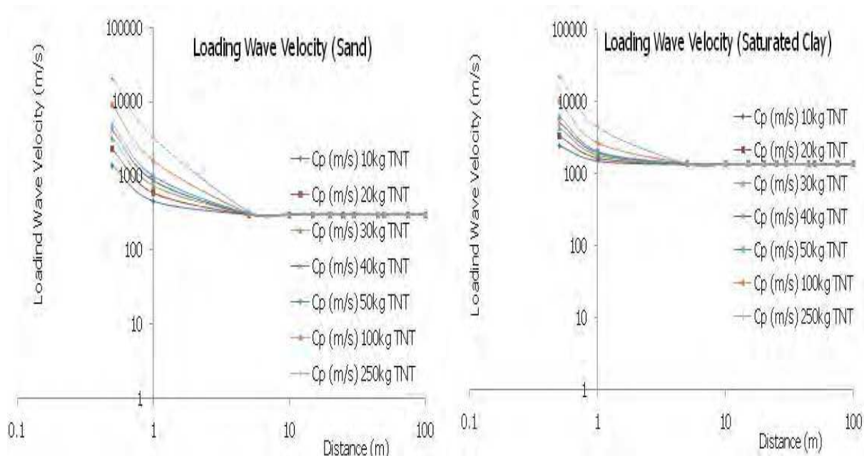
Fig. 3. Loading Wave Velocity for Sand and Saturated Clay for Underground Blast (Olairewaju, et al. 2010c, 2010e, 1020f, 2010i)
