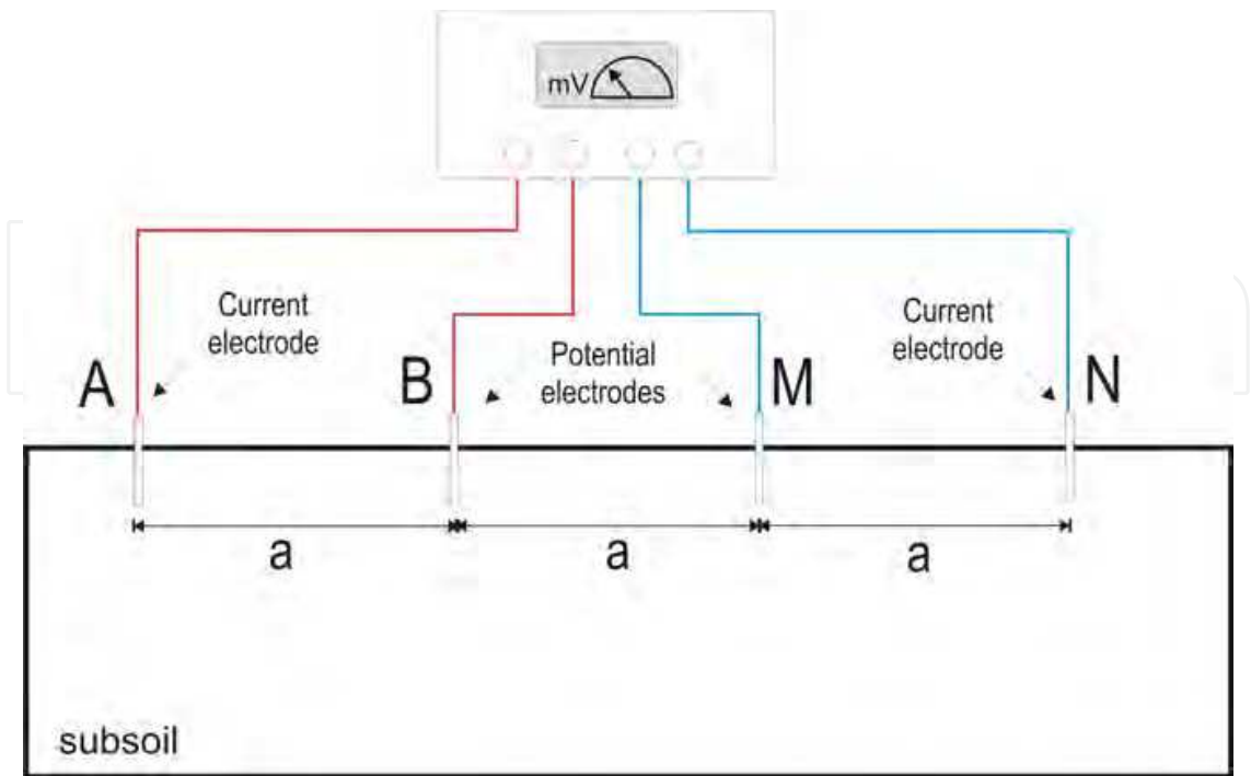
Fig. 10. a) Dipole-dipole array for the acquisition of a measure of electrical resistivity.
