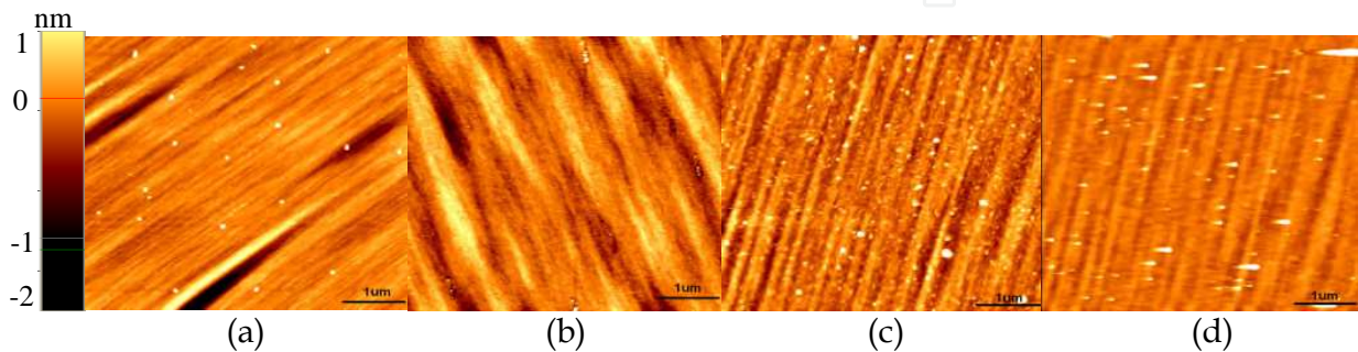
Fig. 6. 5 μm x 5μm AFM micrographs of (a) 6H-SiC, (b) 6H-SiC after alkylation, (c) 6H-SiC APDEMS and (d) 6H-SiC APTES. AFM data taken in tapping mode (Oliveros et al., 2009).
