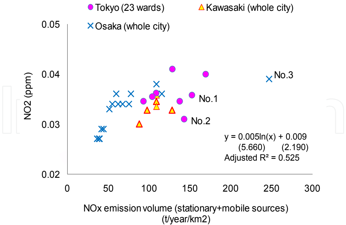
Fig. 6. Correlation between total NOx emissions and NO2 in Tokyo (23 wards), Kawasaki-city, and Osaka-city
