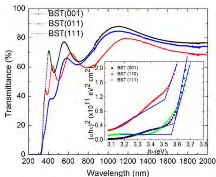
Fig. 2. Optical transmission spectra of [001], [011] and [111]-oriented Ba 0.7 Sr 0.3 TiO 3 thin films. Inset is the plots of (\alpha h\nu)^2 versus h\nu for Ba 0.7 Sr 0.3 TiO 3 thin films. The optical band gap energy E_{\text{gap}} is deduced from extrapolation of the straight line to (\alpha h\nu)^2 = 0 . [Reproduced with permission from Ref. (Wang et al., 2010). Copyright 2010, AIP]
