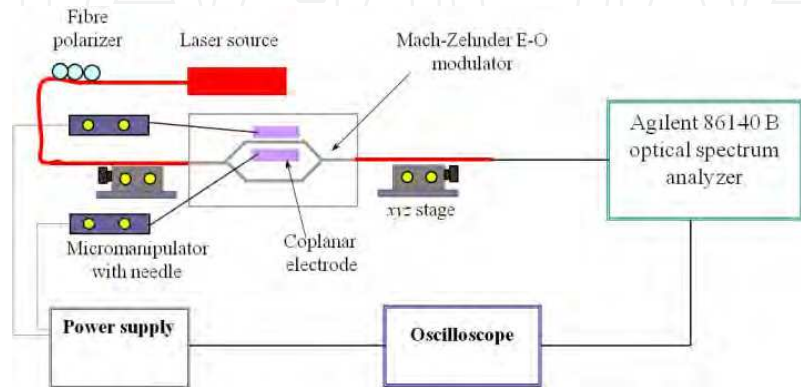
Fig. 19. Experimental setup for the characterization of Mach-Zehnder E-O modulator. [Reproduced with permission from Ref. (Wang et al., 2007b). Copyright 2007, Taylor & Francis]
