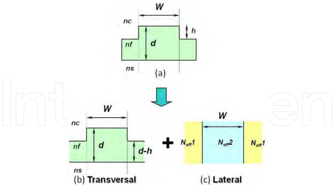
Fig. 12. Description of the effective index method for a rib waveguide. (a) the original rib waveguide; (b) solving the vertical slab problem to define N_{\text{eff1}} and N_{\text{eff2}} ; (c) solving the equivalent horizontal slab problem to determine the N_{\text{eff}} of the whole structure. [Reproduced with permission from Ref. (Wang et al., 2006b). Copyright 2006, Elsevier]
