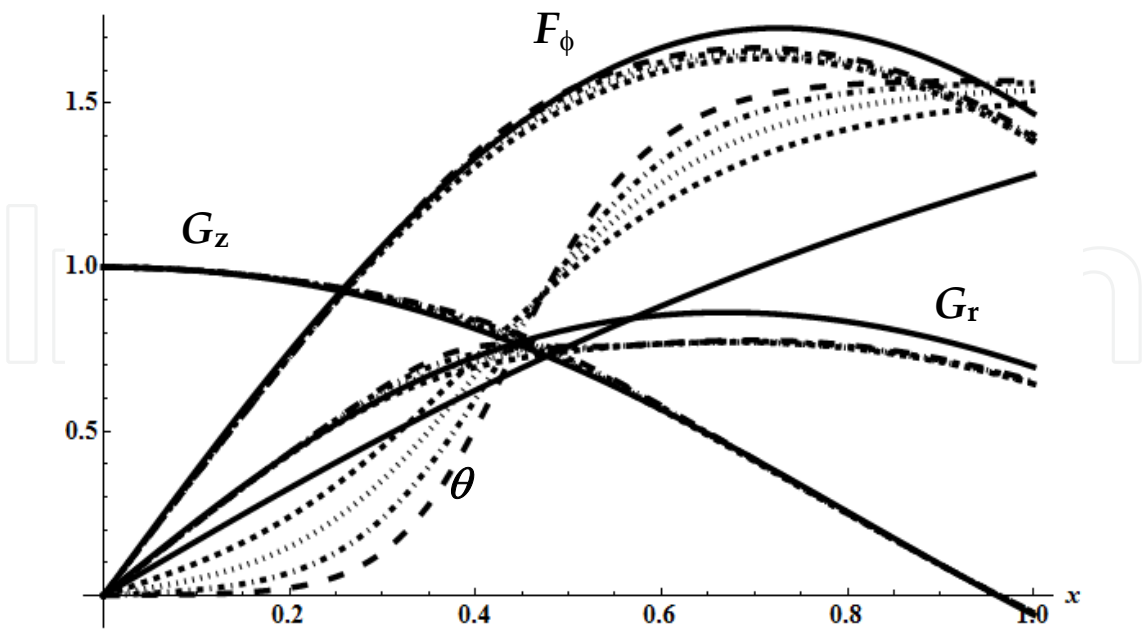
Fig. 8. Dimensionless magnetic and electric fields F_\phi , G_r , G_z and director configuration \theta at the cut-off frequencies, as function of x for five values of q : q = 0 (solid line), q = 50 (dashed line), q = 100 (dotted line), q = 200 (dot-dashed line) and q = 400 (large dashed line).
