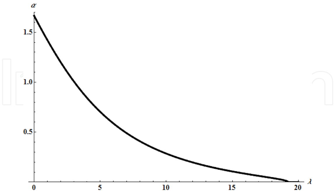
Fig. 3. \alpha = d\theta(0) / dx against \lambda for the first fourth modes. These modes coincide for each of the values of \lambda .
