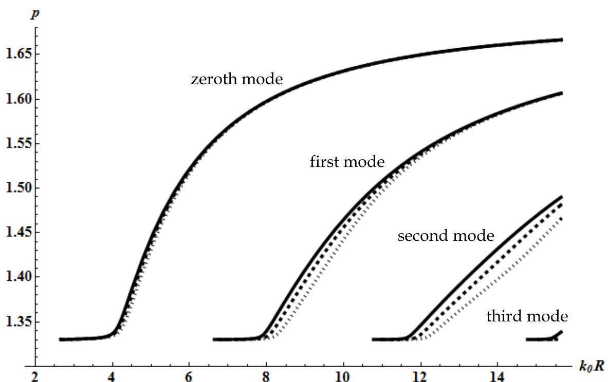
Fig. 10. Dispersion relation p vs k_0 R for the first four modes at intensities \lambda = 0 (solid line), \lambda = 2 (dashed line) and \lambda = 4 (dotted line). The minimum value of vertical axis takes places at p = n_c = 1.33 .
