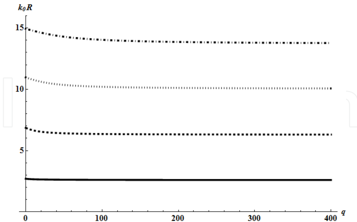
Fig. 6. Cut-off frequencies k_0 R for the zeroth (solid line), first (dashed line), second (dotted line) and third (dot-dashed line) modes versus q . As it can be seen, the cut-off frequencies k_0 R gets smaller as optical intensity parameter q gets larger.
