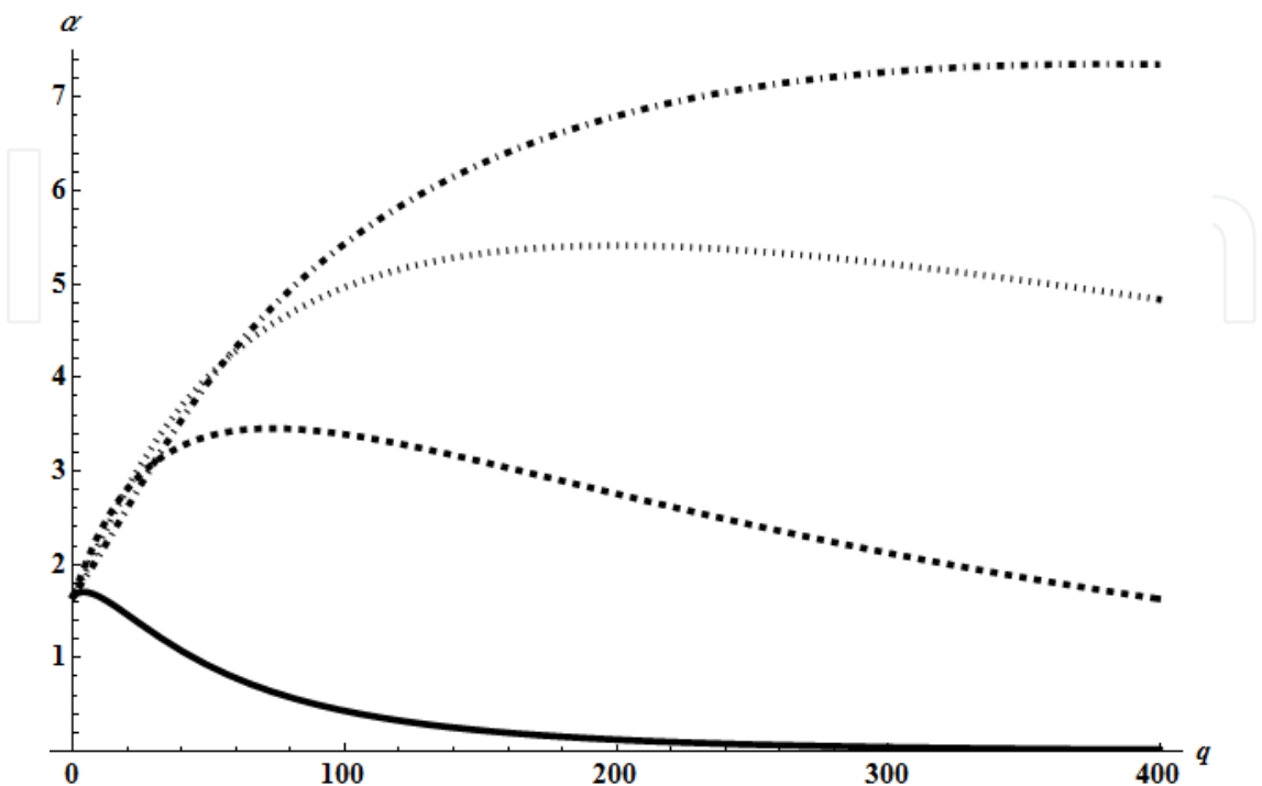
Fig. 7. \alpha = d\theta(0) / dx against q for the same modes of Fig. 6. Notice that, when the electromagnetic field is absent, q = 0 , we obtain only one value for \alpha = d\theta(0) / dx , in agreement with Fig. 3.
