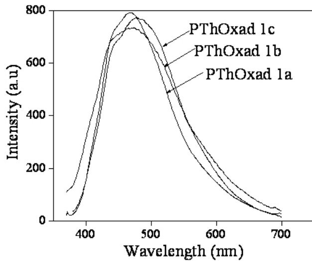
Fig. 7. Fluorescence emission spectra for PThOxad 1a-c in DMF solution.
