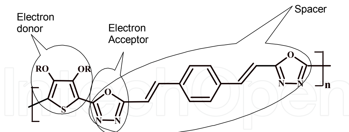
Fig. 1. Chemical structures of donor-acceptor conjugated polymers, PThOxd 1a-c, showing donor, acceptor and spacer units.
