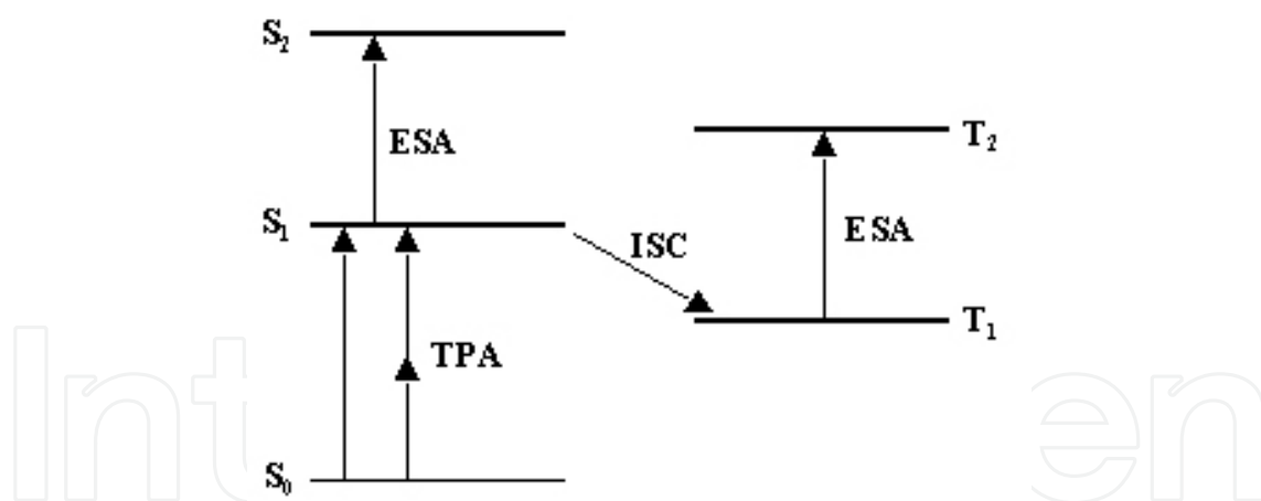
Fig. 14. Energy level diagram showing both two-photon absorption and excited state absorption.
