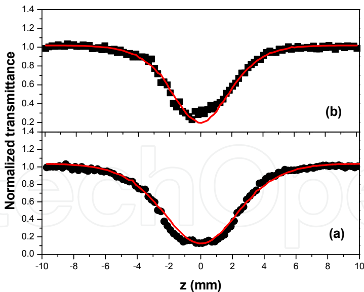
Fig. 22. Open aperture z-scan of nanocomposite films having a linear transmission of 51 % at 532 nm. The laser pulse energy is a) 100 microJoules, b) 75 microJoules. Circles are data points while the solid curve is a numerical fit according to equation (6).
