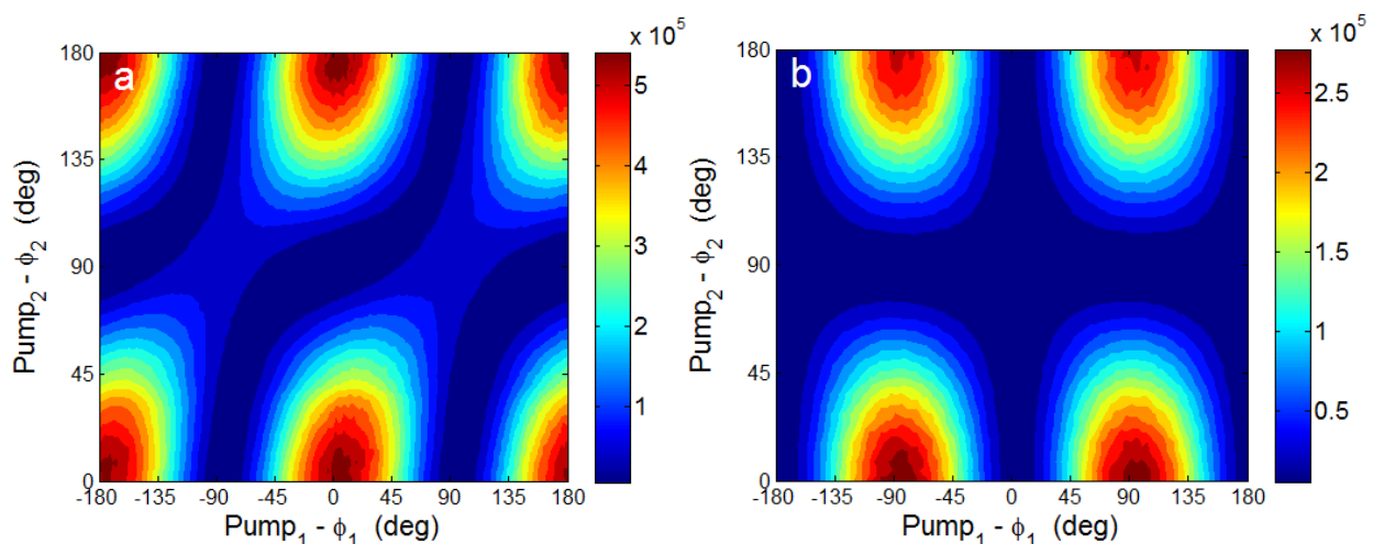
Fig. 5. Noncollinear second harmonic signal experimentally measured as a function of the polarization state of the first pump beam ( \phi_1 ) and the second pump beam ( \phi_2 ). Sample rotation angle was fixed to \alpha=9^\circ . The polarization state of the analyzer is set to (a) \hat{p} i.e. \phi=0^\circ and (b) \hat{s} , i.e. \phi=90^\circ .
