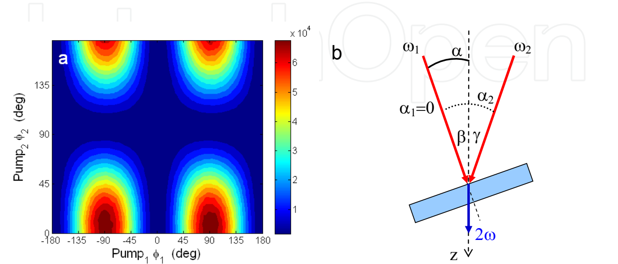
Fig. 6. (a) Noncollinear SH signal measured as a function of the polarization state of the first pump beam ( \phi_1 ) and the second pump beam ( \phi_2 ). The polarization state of the analyzer is set to \hat{s} , i.e. \phi=90^\circ . (b) Sketch of the experimental configuration: sample rotation angle was fixed to \alpha=9^\circ .
