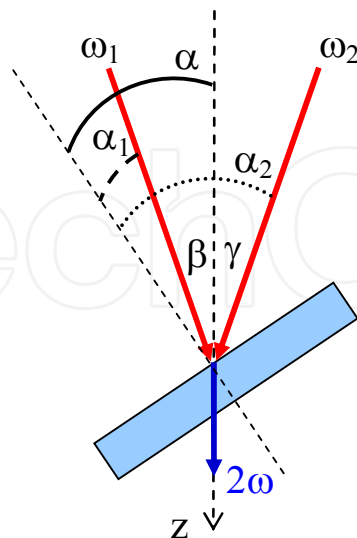
Fig. 1. Sketch of the noncollinear scheme adopted for second harmonic generation measurements. For a fixed sample rotation angle \alpha , measured with respect to the z-axis, the corresponding incidence angles of the two pump beams result to be \alpha_1 = \alpha - \beta and \alpha_2 = \alpha - \gamma , respectively.
