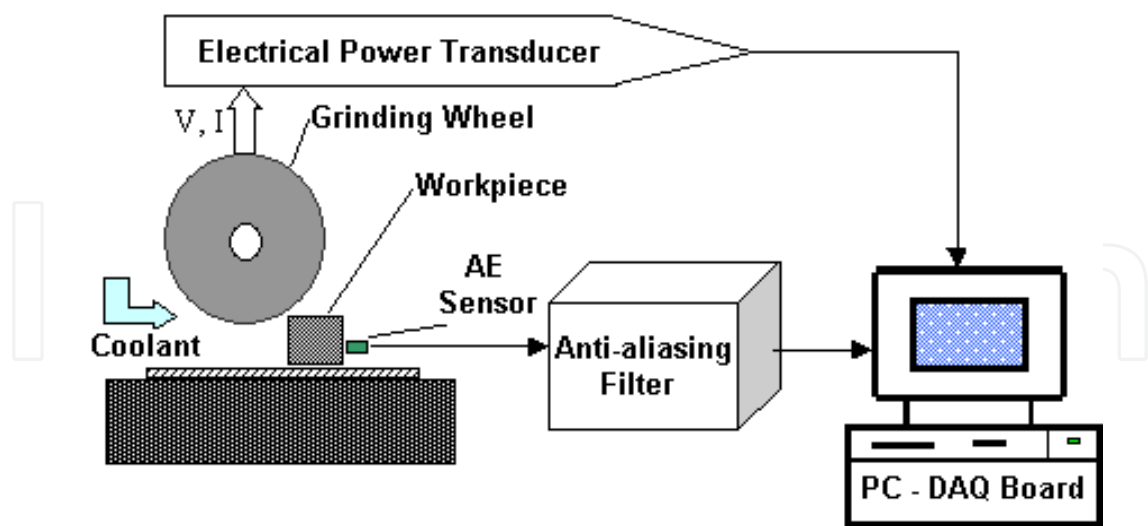
Fig. 1. Experimental setup
