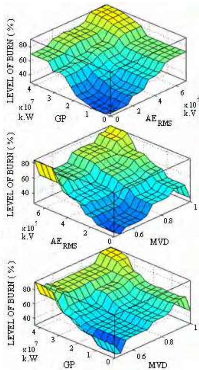
Fig. 10. 3D analysis of the surface generated by the rules system of model 2
