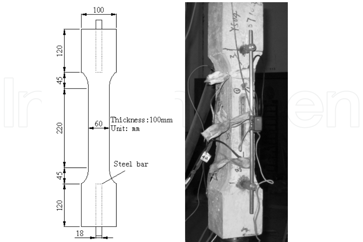
Fig. 1. Dimension and shape of concrete specimens
