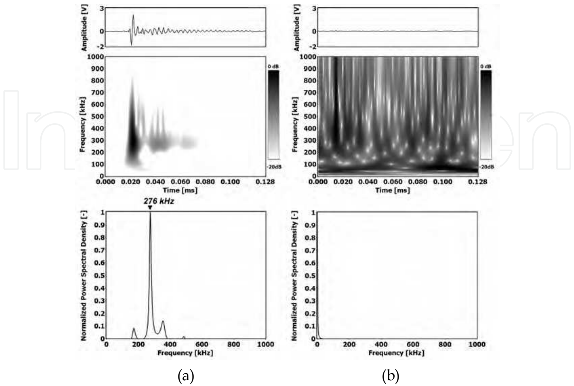
Fig. 14. Time waveform, continuous wavelet transform (CWT) spectrogram and normalized MUSIC power spectrum density prepared for acoustic emission signals generated by partial discharges in internal gas void (PD4), which were registered with wideband sensor type WD (a) and narrowband sensor type D9241A (b)
