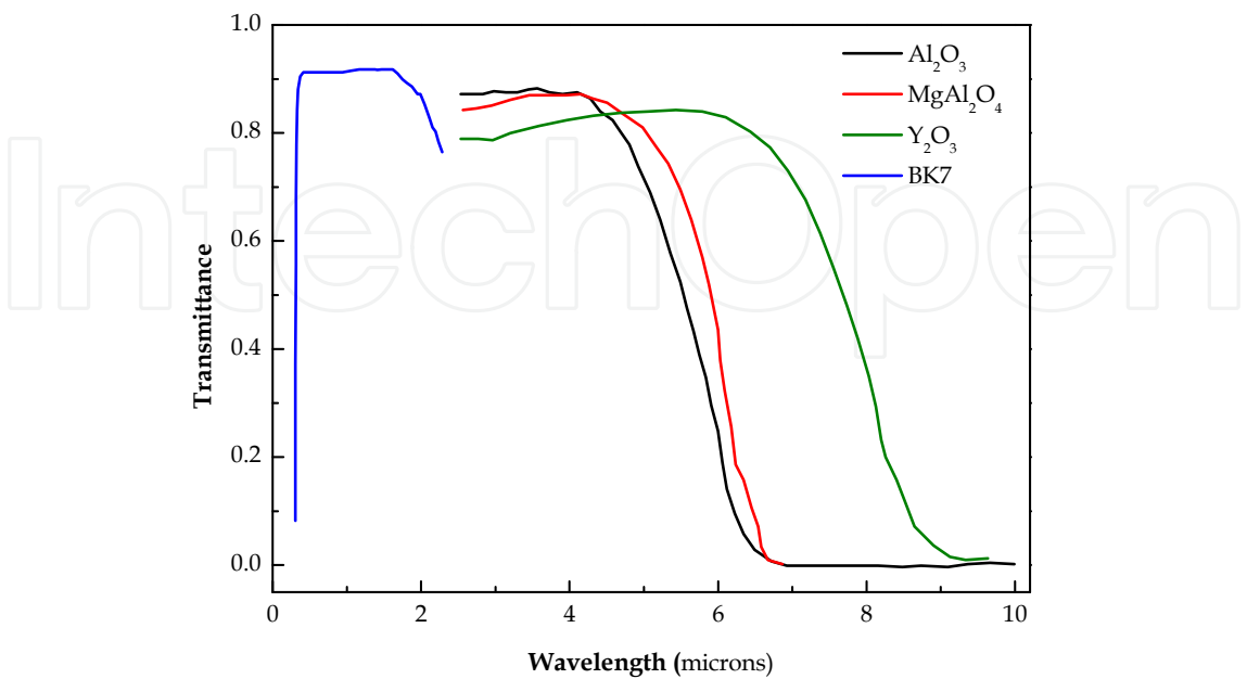
Fig. 1.2. Transmittance spectra of different materials.
