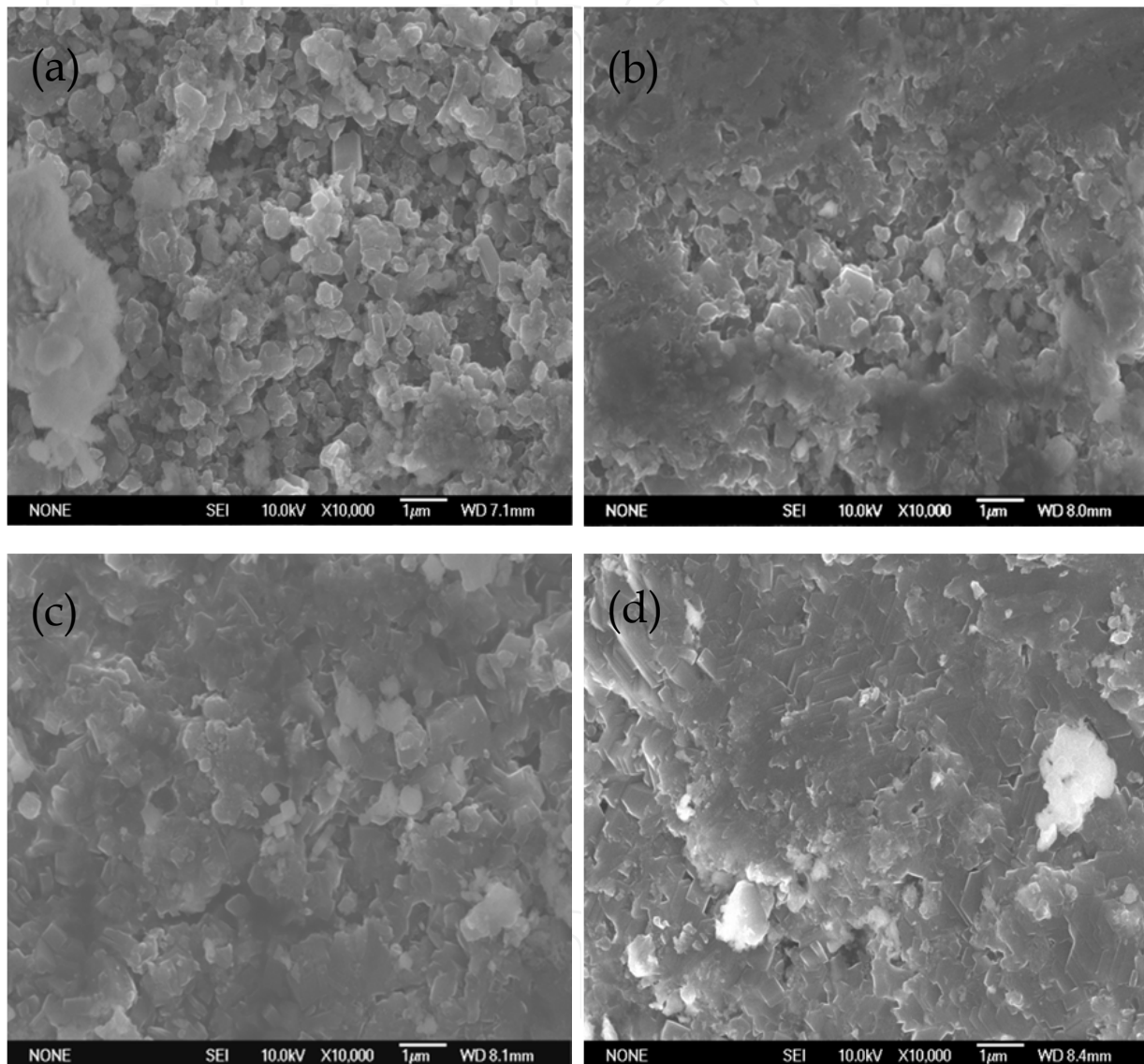
Fig. 9. SEM images of the microstructures of the (\text{Mg}_{1.1}\text{B}_2)_{1-x}\text{Cu}_x samples sintered at 575 °C for 5 h with (a) x = 0.0 , (b) x = 0.03 , (c) x = 0.05 and (d) x = 0.10 , respectively [42].
