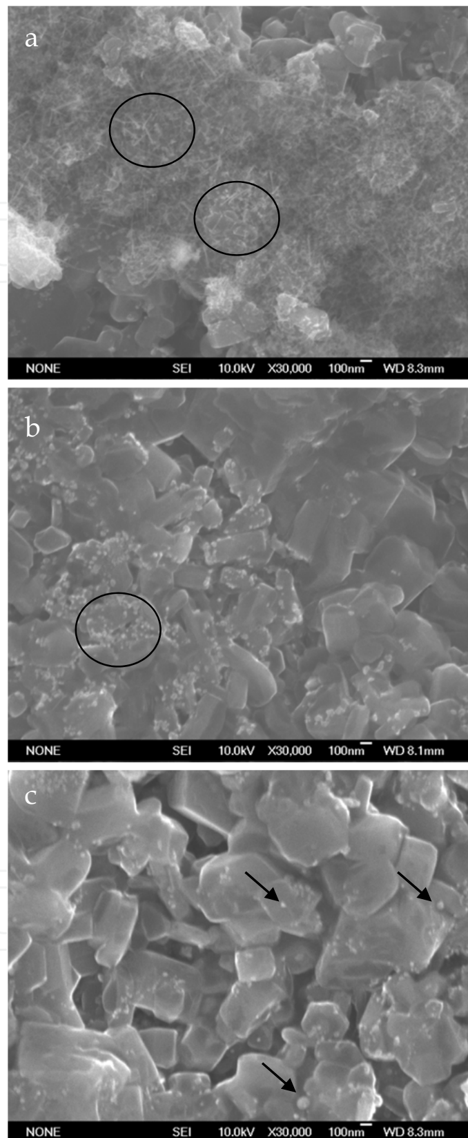
Fig. 17. Scanning electron microscopy images of the (\text{Mg}_{1.1}\text{B}_2)_{1-x}\text{Cu}_x samples sintered at 850^\circ\text{C} for 30 min with (a) x = 0 , (b) x = 0.01 and (c) x = 0.03 , respectively. The MgO whiskers and nanoparticles are indicated by the black circles and arrows in the figures [51].
