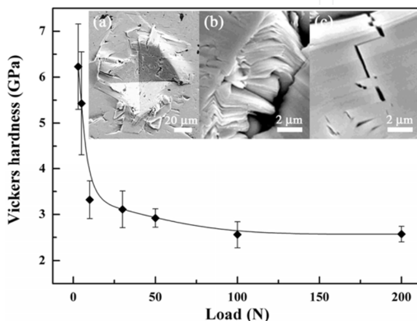
Fig. 7. Vickers hardness of \text{Nb}_4\text{AlC}_3 as a function of indentation loads. The insets show (a) push-out, (b) delamination, kink, and basal plane slips, and (c) zigzag crack propagation in a grain in an indent under a load of 10 N [4].
