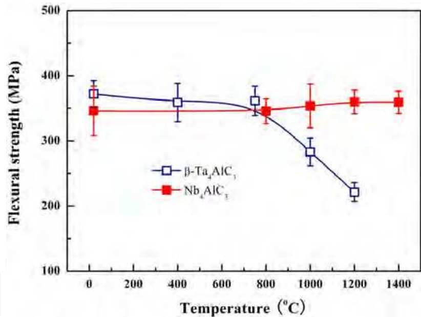
Fig. 9. Temperature dependent flexural strength of \text{Nb}_4\text{AlC}_3 and \beta\text{-Ta}_4\text{AlC}_3 [4].
