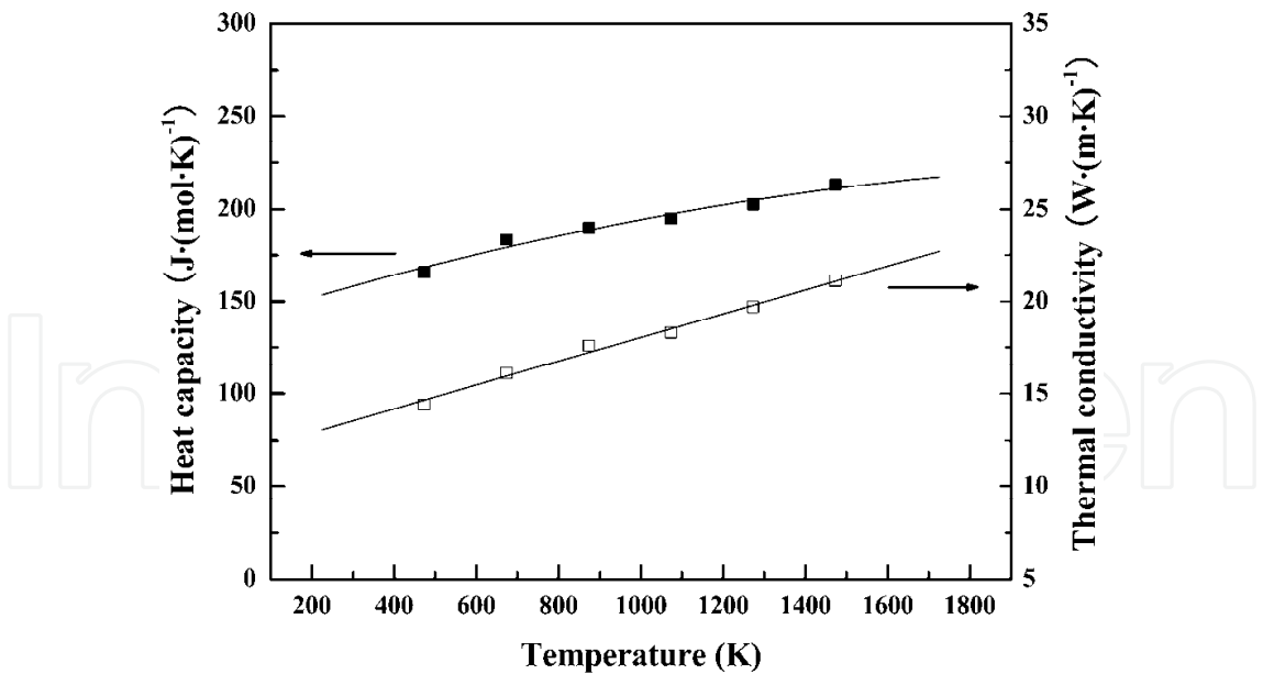
Fig. 6. Temperature dependences of molar heat capacity and thermal conductivity of \text{Nb}_4\text{AlC}_3 [4].
