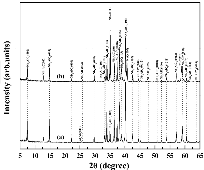
Fig. 13. Effect of holding time on the synthesis of Nb 4 AlC 3 : (a) 2 minutes and (b) 4 minutes [5].
