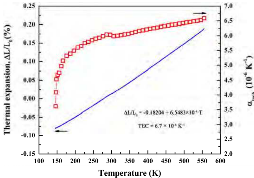
Fig. 16. Temperature dependence of thermal expansion and technical thermal expansion coefficient of Nb 4 AlC 3 in a temperature range of -128 and 282°C [5].
