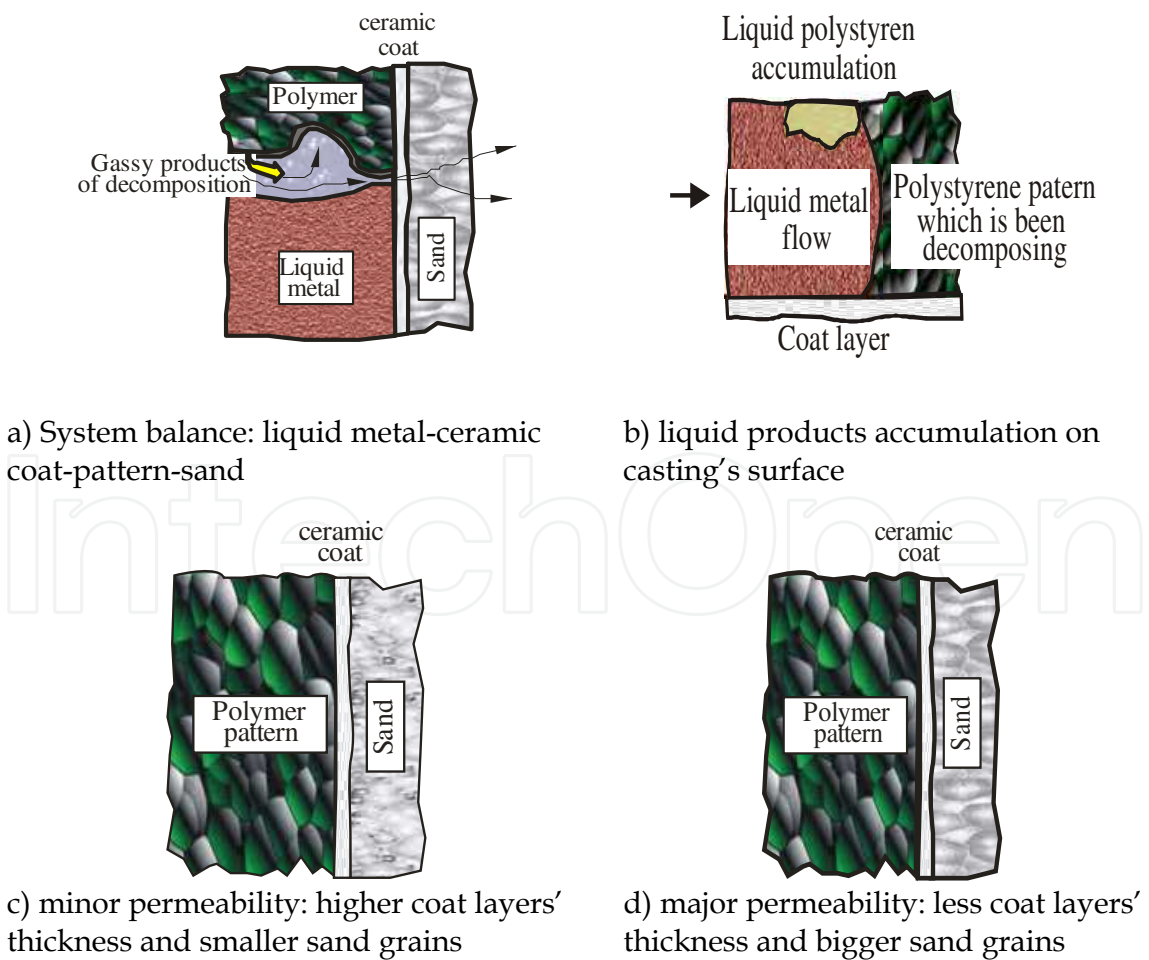
Fig. 4. EPC process: The role of ceramic coating
