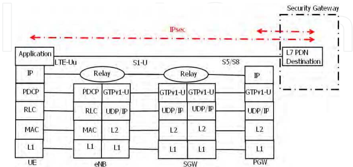
Fig. 5. IPsec scheme in LTE topology
