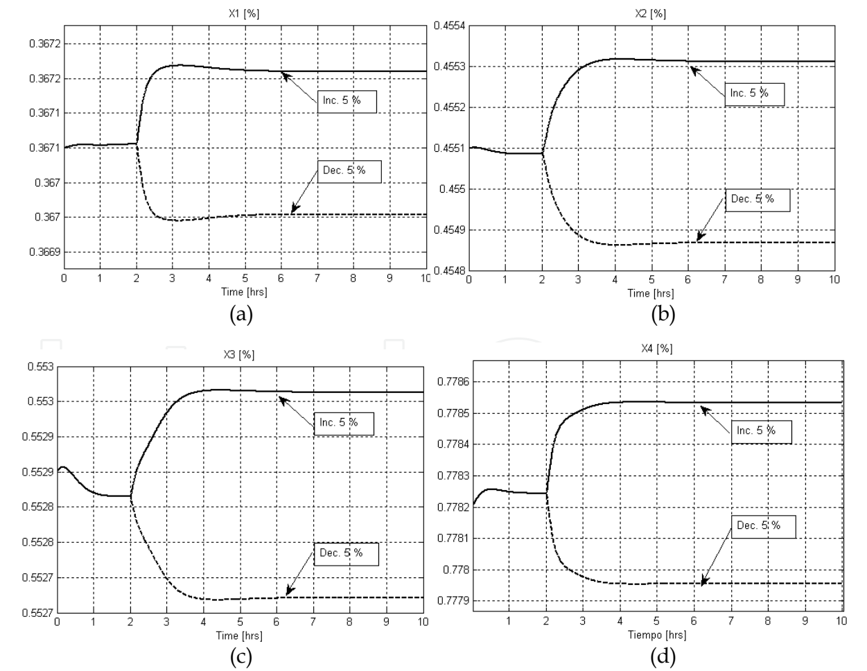
Fig. 9. Behavior of the concentration in the evaporator to a change of a step in the temperature of the input solution (increase of 5% - decrease of 5%).
