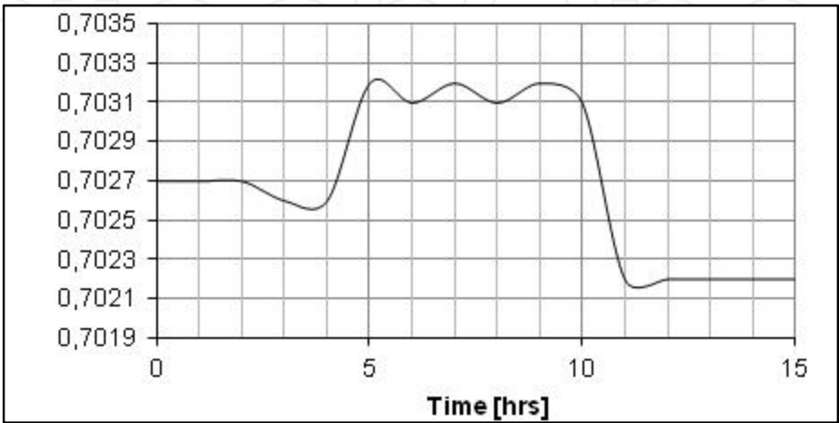
Fig. 11. Behavior of the final product concentration at the outlet of the fourth effect
