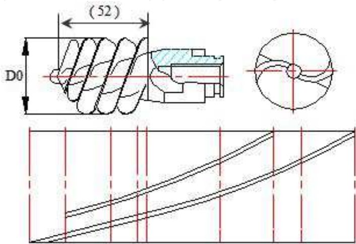
Fig. 4. Inducer with two long and two short blades
