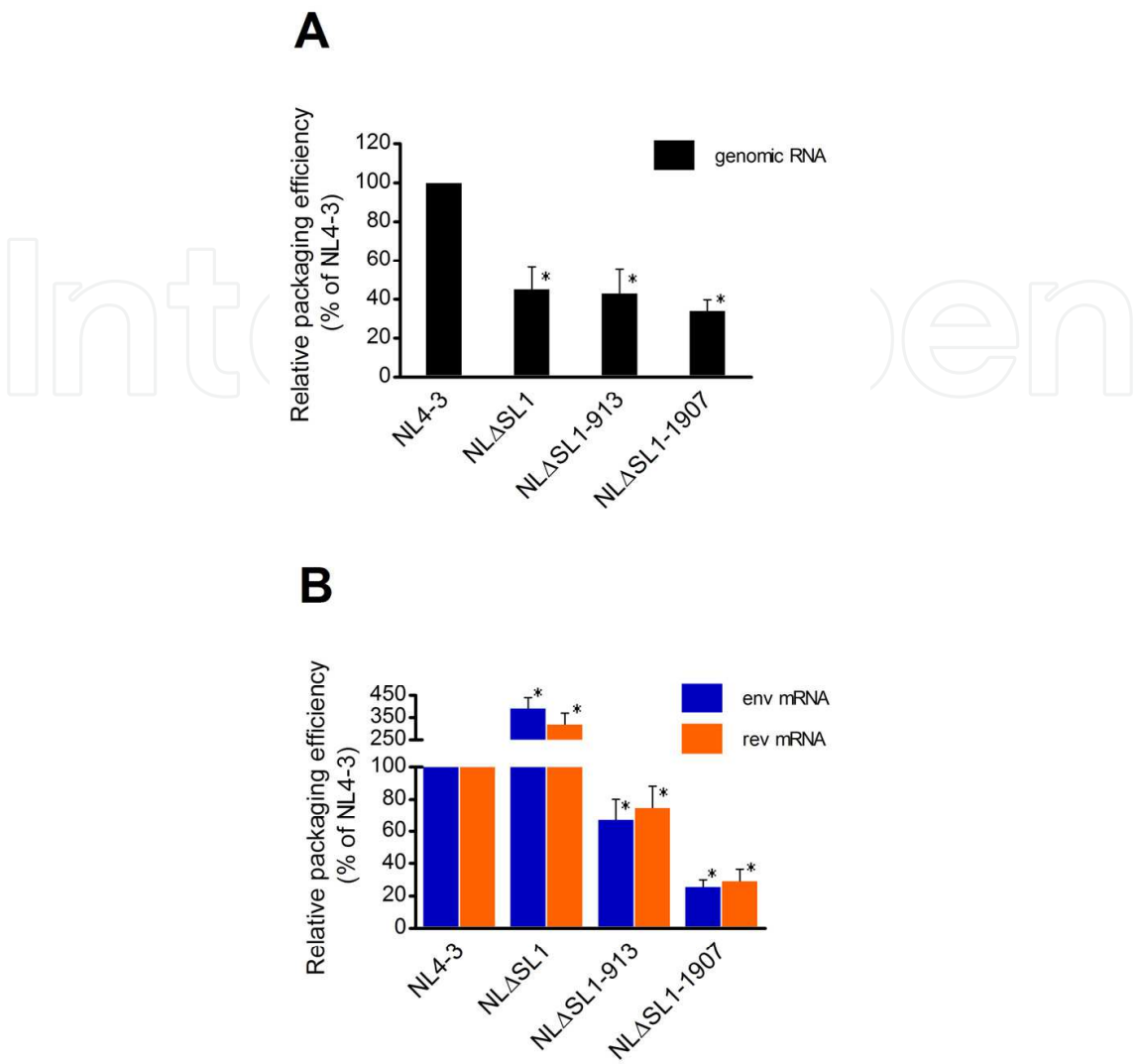
Fig. 4. Quantification of HIV-1 RNA content in the virion by real-time PCR. (A) Efficiency of HIV-1 genomic RNA packaging. NL4-3, wildtype HIV-1; NLΔSL1, SL1 deletion mutant; NLΔSL1-913, ΔSL1 with compensatory mutation in matrix; NLΔSL1-1907, ΔSL1 with compensatory mutation in SP1. The amount of NL4-3 genomic RNA was set at 100%. *, indicates p < 10^{-4} and significant deviation from the wild-type copy number as determined by Student's t test. (B) Efficiency of spliced HIV-1 RNA (env and rev mRNA) packaging. The amount of NL4-3 spliced mRNA was set at 100%. *, indicates significant deviation from the wild-type copy number as determined by Student's t test; p < 10^{-4} , except for NLΔSL1-913, p < 10^{-3} .
