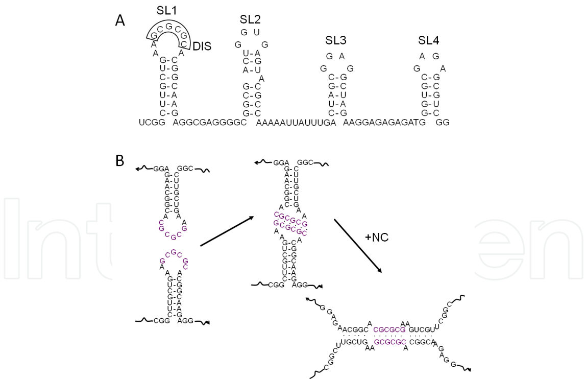
Fig. 3. Stem-loops of the HIV-1 5' untranslated region. (A) RNA structure of the four stem-loops. The dimerization initiation signal (DIS) sequence is shown in box. (B) Mechanism of viral RNA dimerization. Dimerization is initiated by base-pairing of the DIS forming a kissing-loop complex. Gag nucleocapsid (NC) promotes the formation of a more stable RNA dimer.
